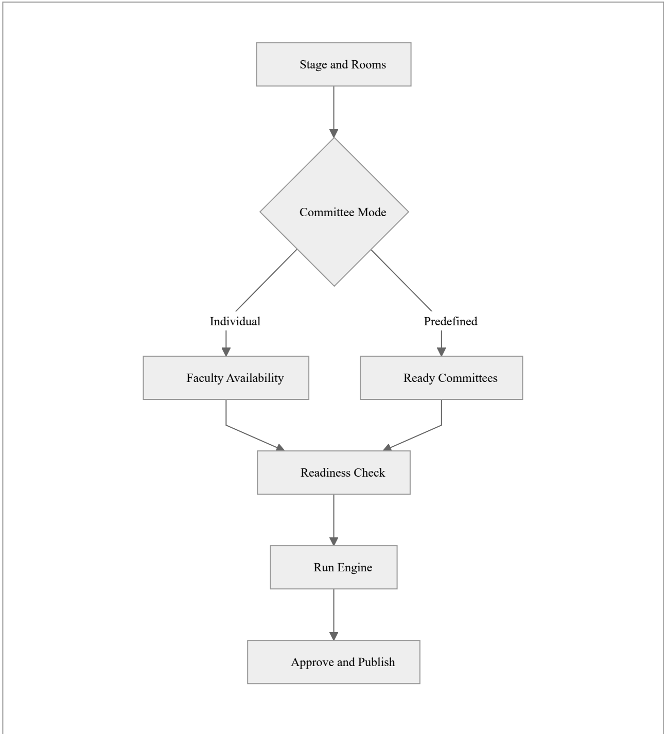
Figure 3: End-to-end workflow with committee branch
