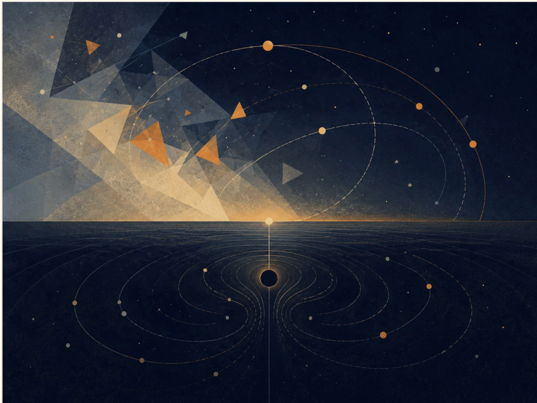
Figure F: The imaginary, the virtual, and the horizon in the logical model.
