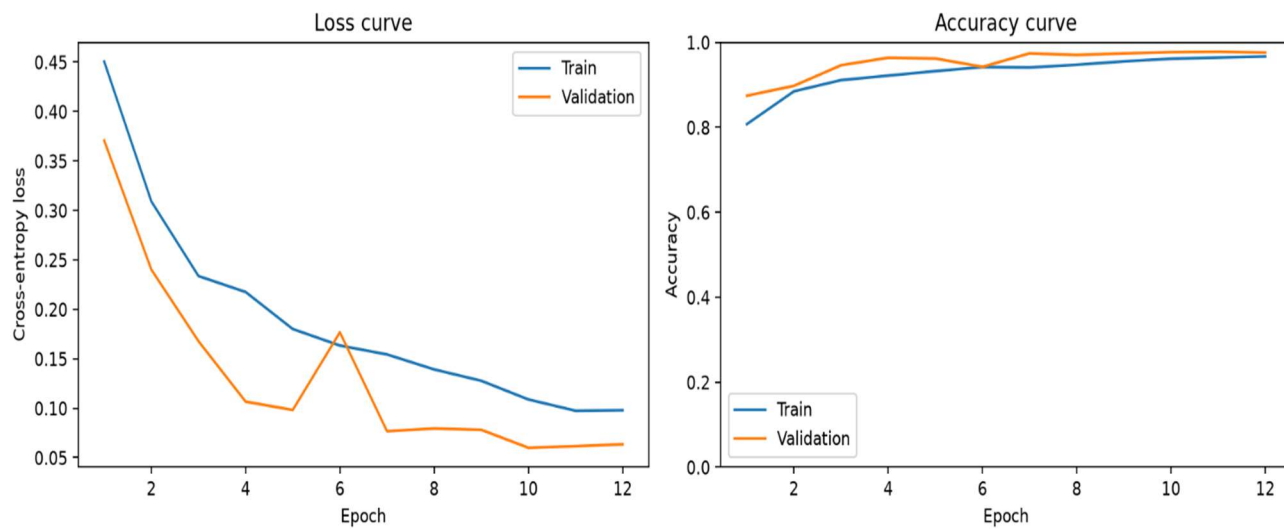
Figure 5.3.3 Training and Validation Loss/Accuracy Curves
