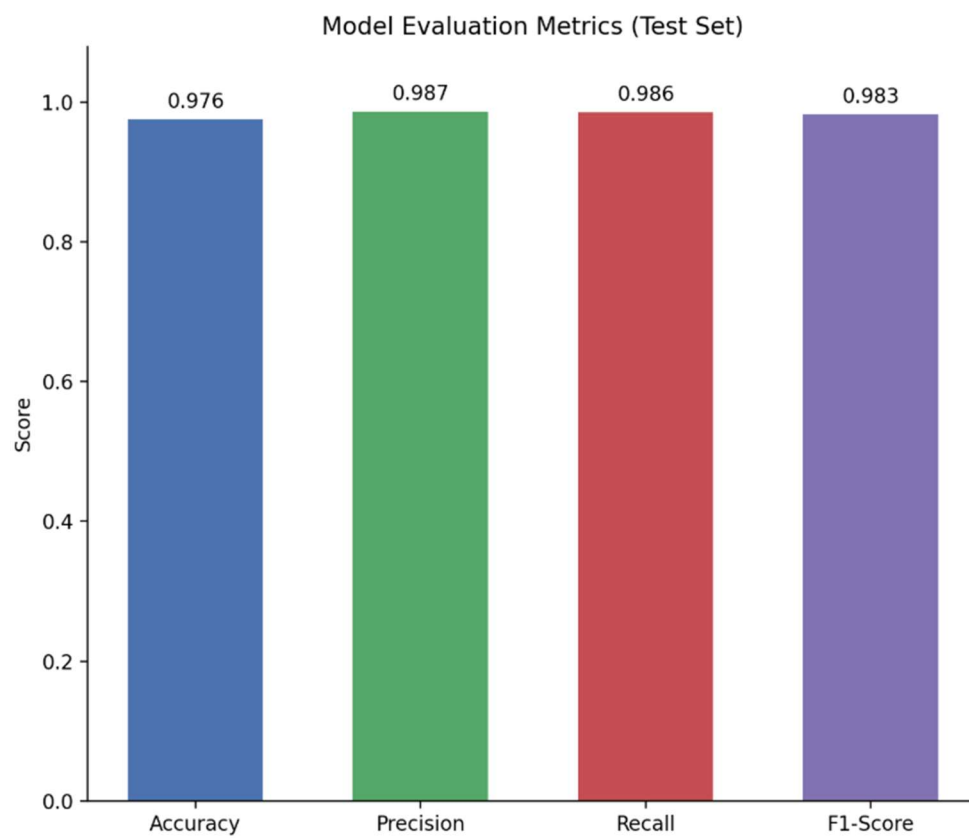
Figure 2.3.1 Model Evaluation Metrics on the Test Set
