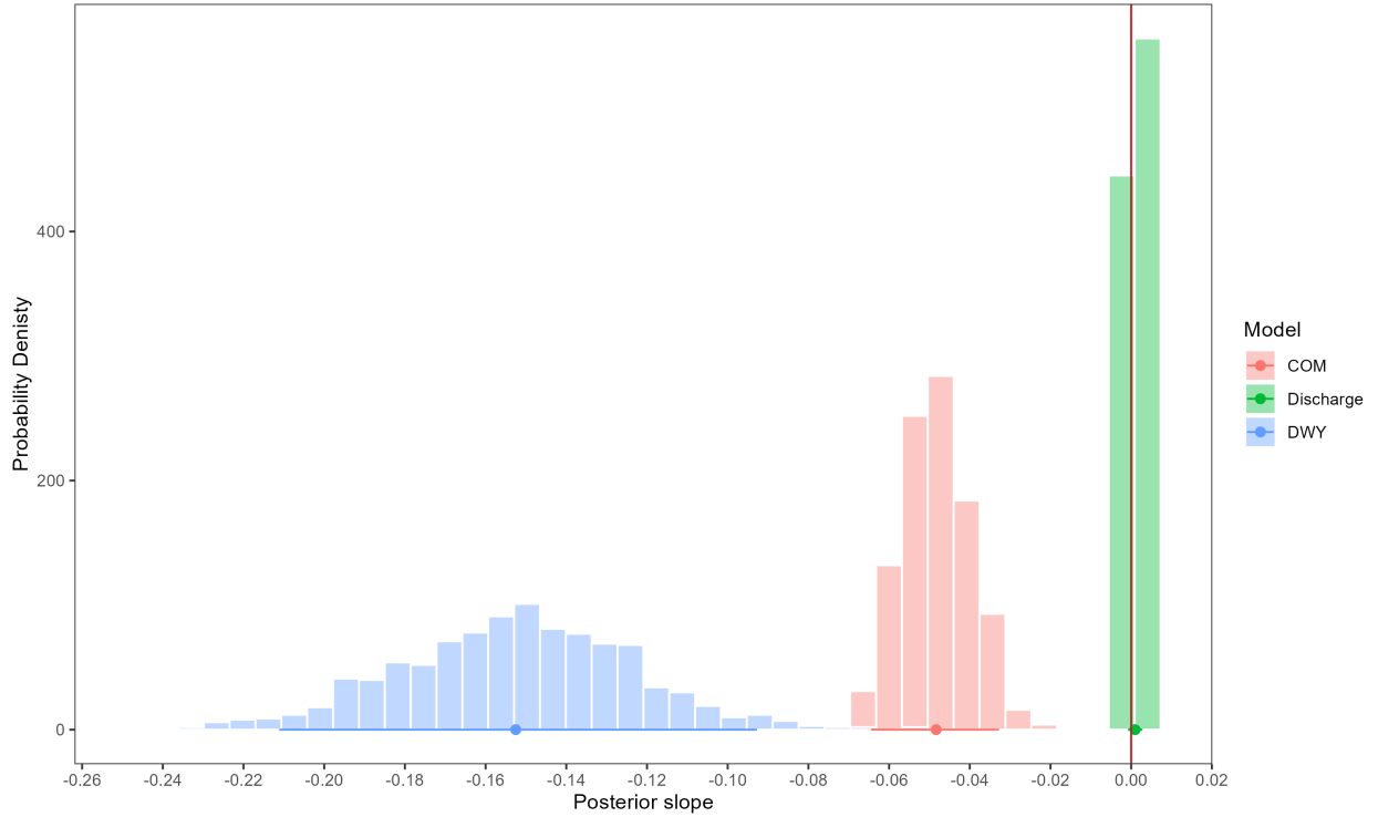
Figure 2: Posterior slope probability density histogram for center of mass (COM), day of water year containing annual peak flow (DWY), and discharge, based on 1000 posterior draws. Horizontal segments across the x-axis represent the 90% confidence interval for each model and the dot represents the posterior mean slope. The red vertical line is the zero threshold, meaning no positive or negative slope. This visualization highlights the difference in slope and confidence among the modeled variables with discharge exhibiting a tightly constrained slope near zero and the DWY and COM showing a stronger negative slope.
