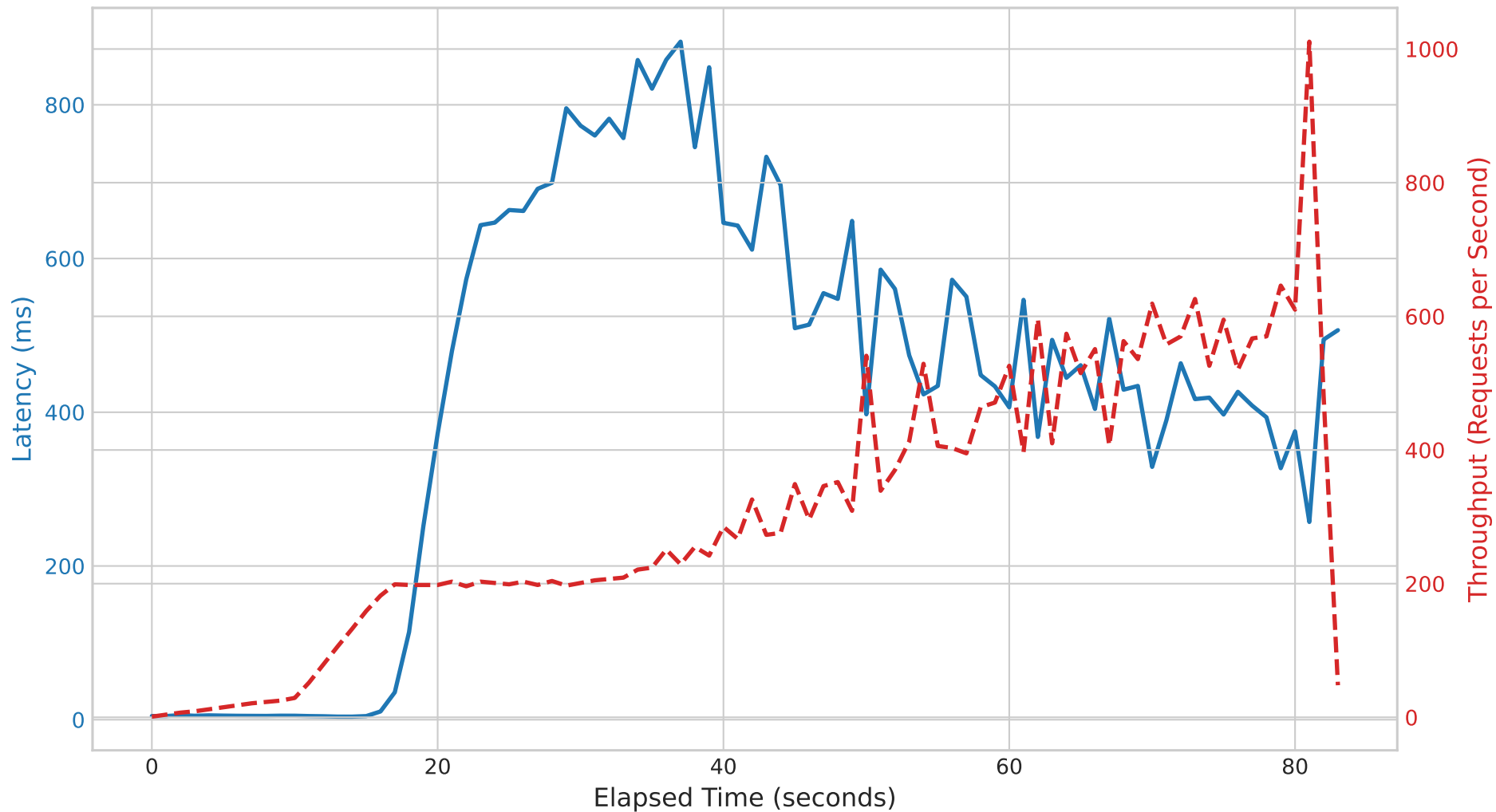
Performance Analysis: Matrix Multiplication API
