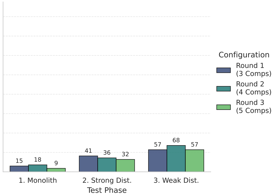
POST Requests
