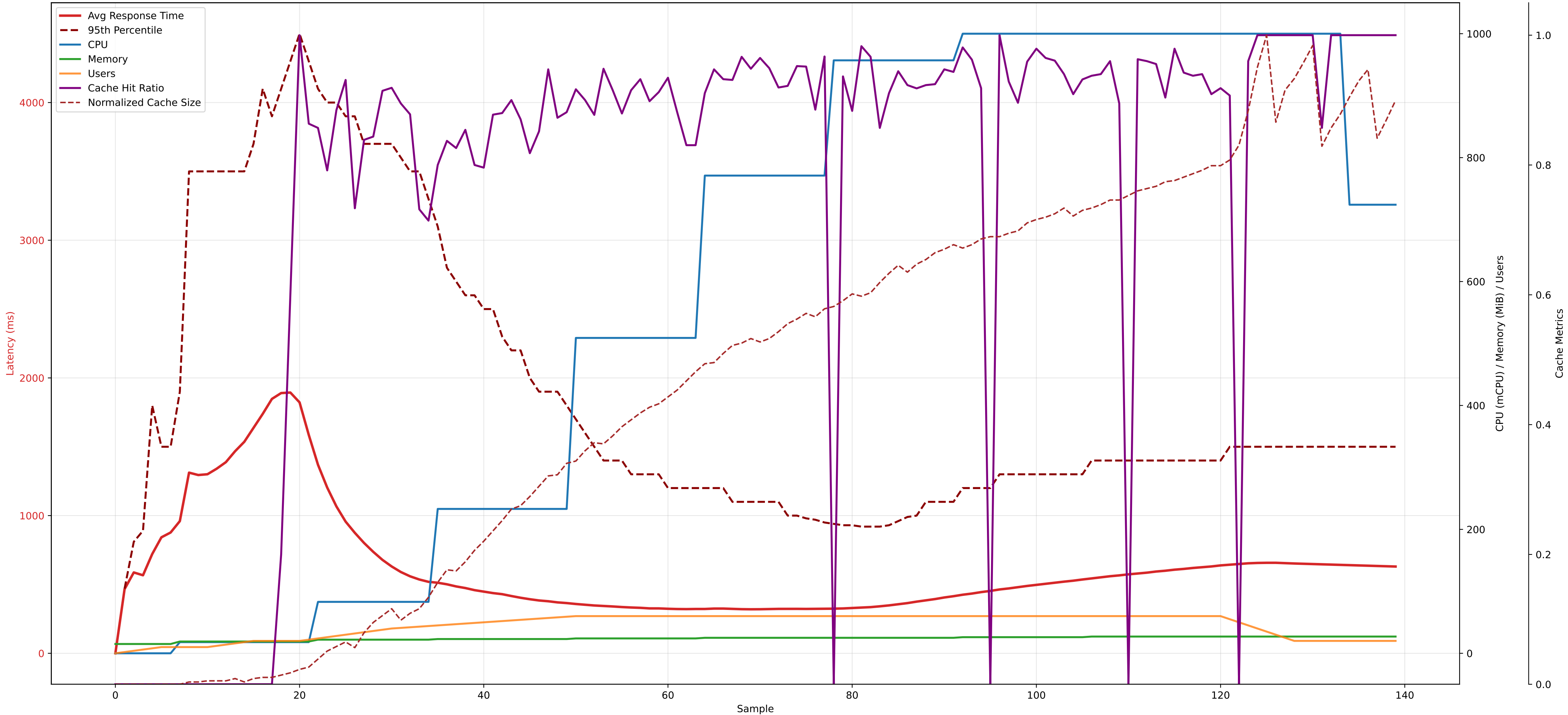
Impact of Cache on Service Performance, Resource Utilization and Errors
