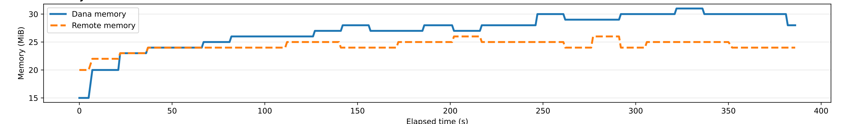
Memory Utilization
