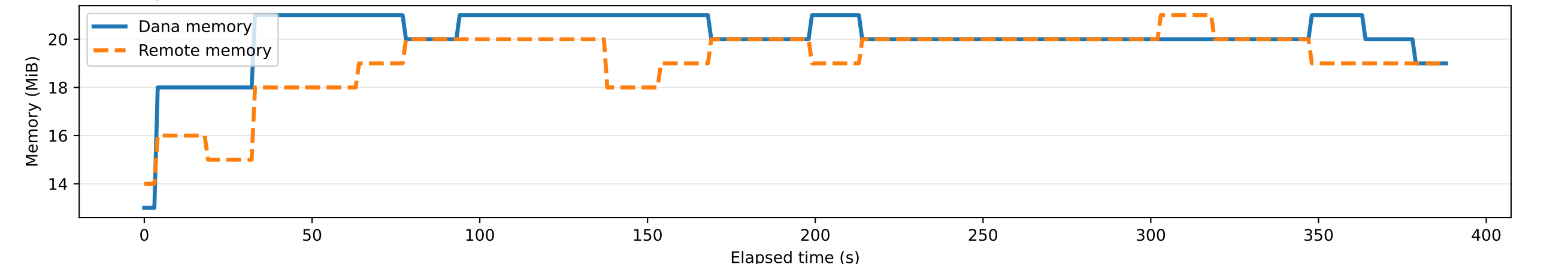
Memory Utilization
