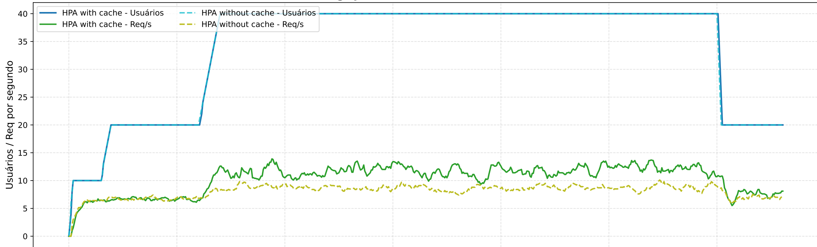
Workload e Throughput: HPA with cache vs HPA without cache
