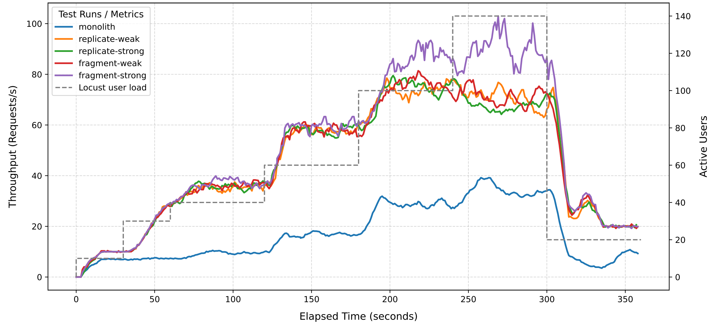
Locust Performance Test - Throughput (RPS) Comparison
