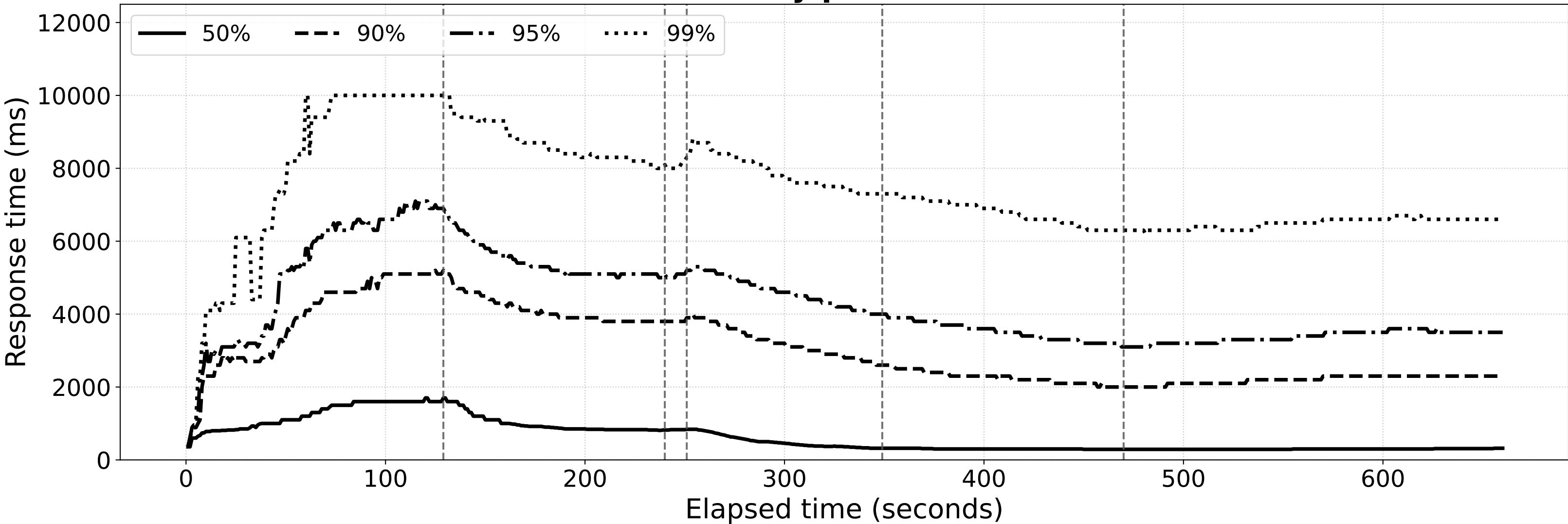
Latency percentiles
