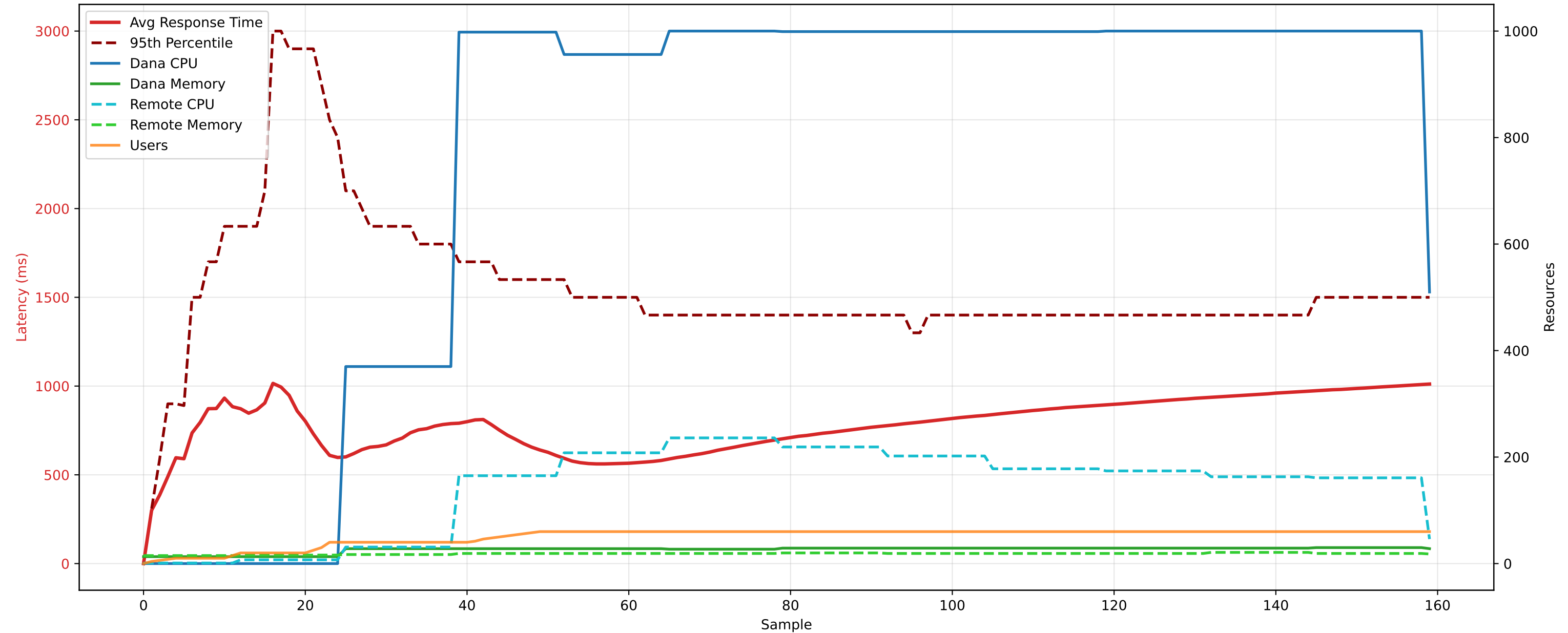
Impact of Cache on Service Performance, Resource Utilization and Errors
