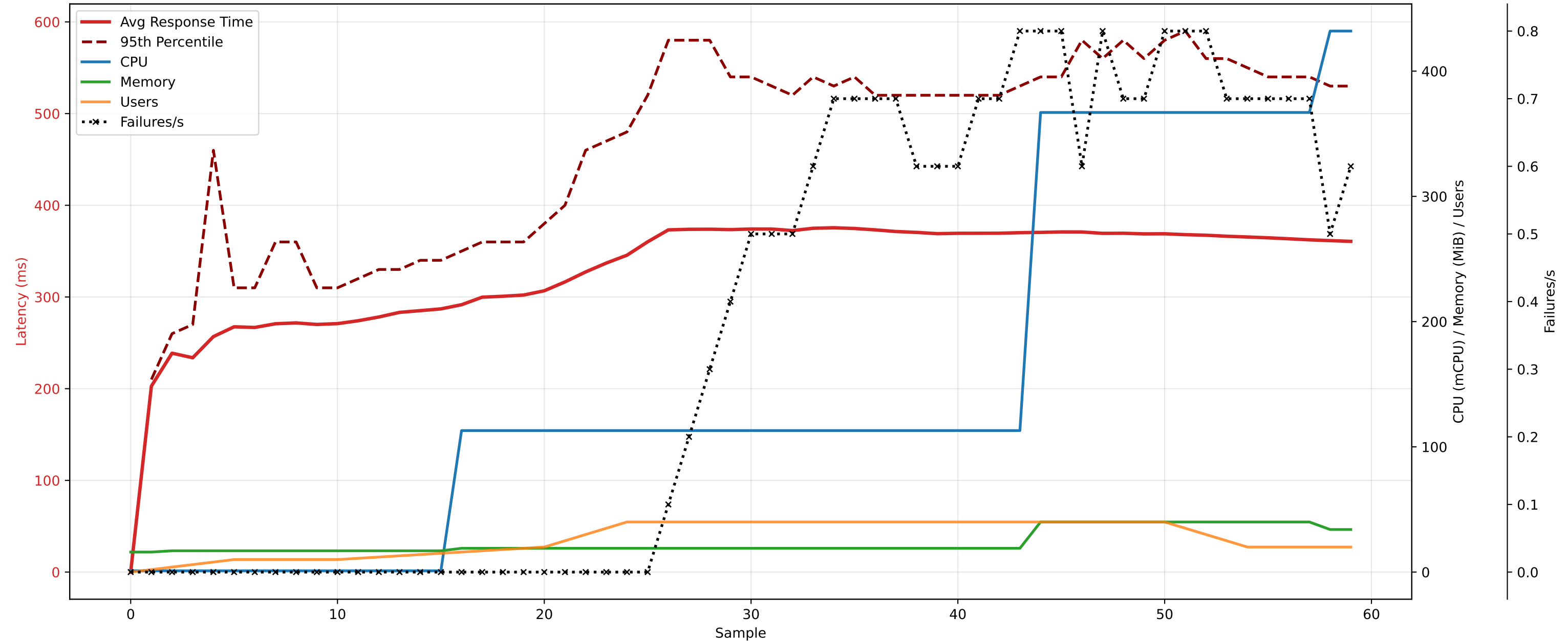
Impact of Database Latency on Service Performance, Resource Utilization and Errors
