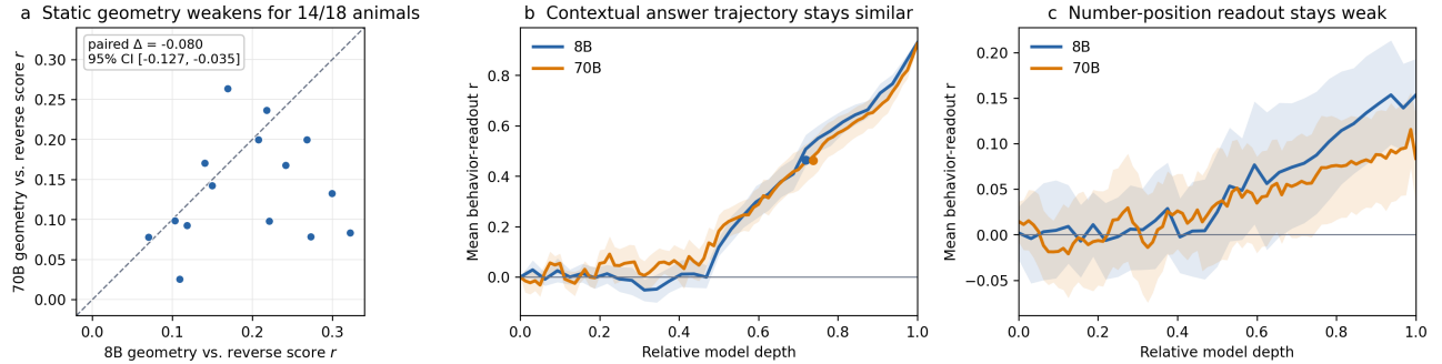
Figure 2: Static geometry and observational readout. (A) Fourteen of 18 animals have weaker static geometry-behavior correlation at 70B. (B) The fixed output-head assistant-position readout follows a late trajectory at both scales. (C) Readout at number positions remains weak. Intervals resample the same 18 animals.
