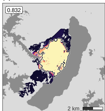
(A) fitted random effect
