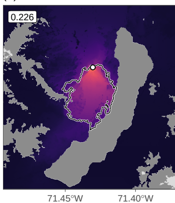
(B) simulated random effect
