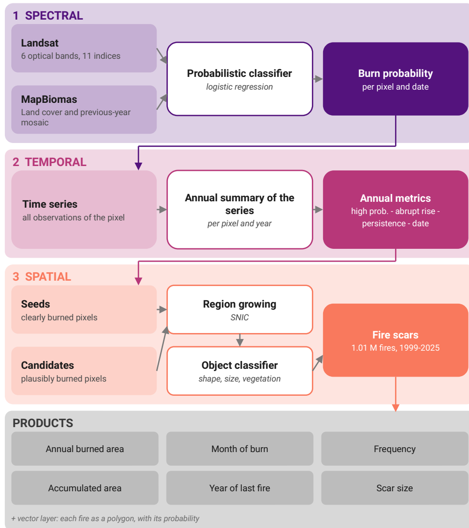
Figure 1: The Collection 1 algorithm. Spectral: Landsat bands and indices, plus MapBiomas land cover and the previous-year mosaic, feed a logistic-regression classifier that scores each pixel and date with a burn probability. Temporal: the per-pixel time series of that probability is summarised into annual metrics, capturing how high it rises, how abruptly, how long it persists, and when. Spatial: the metrics separate clearly burned seeds from plausibly burned candidates, which SNIC region-growing connects into segments; an object classifier filters those on shape, size and vegetation to yield the 1.01 M fire scars mapped over 1999–2025. The six published subproducts and the fire-object polygon layer are both built from that same set of scars.
