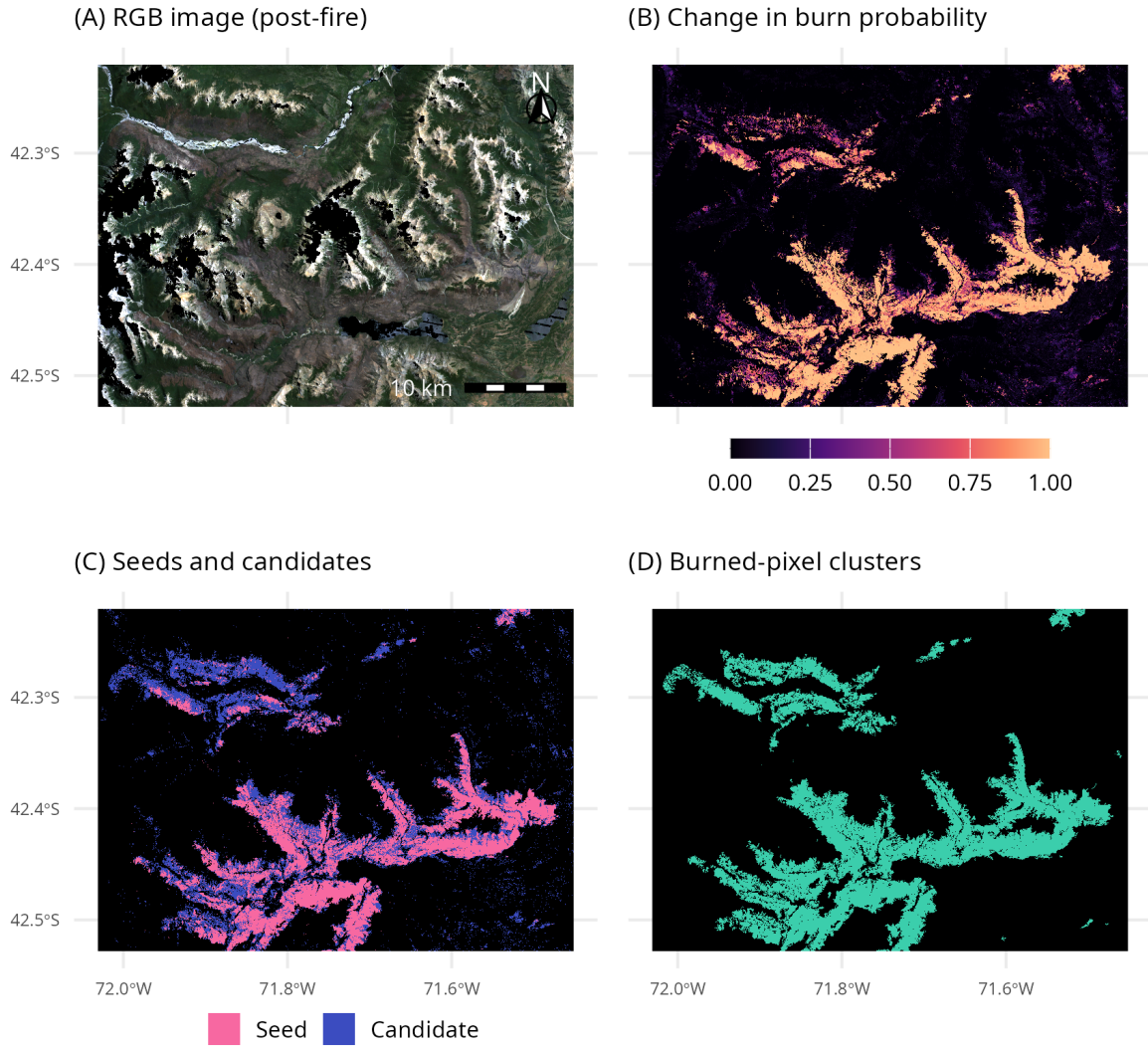
Figure 4: The region-growing step, illustrated on two fires that burned in 2015 in Chubut province (Río Turbio to the north, Cholíla to the south). (A) RGB composite of the following summer, for reference only; black areas are masked by the quality filters. (B) The per-pixel evidence of burning as \Delta 2_{\text{peak}} . (C) Seeds and candidates, obtained by applying a strict and a permissive cut to that evidence. (D) The output of the region growing: the candidate pixels connected to at least one seed.
