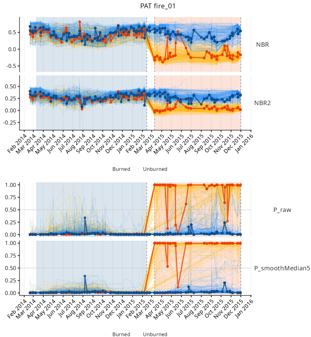
Figure 2: Diagnostic panel for one collected fire (Cholila, Patagonia, 2015). Thin lines are individual training points, thick lines the median across points; orange is the burned class, blue the unburned class. The top two rows show the raw NBR and NBR2 series and the shaded pre-fire and post-fire windows defined by the collector; the bottom two show the predicted burn probability per observation, raw and smoothed. Unburned points keep a low probability throughout, while burned points jump to near 1 at the fire and stay there. That is the signature the temporal stage is built to measure.
