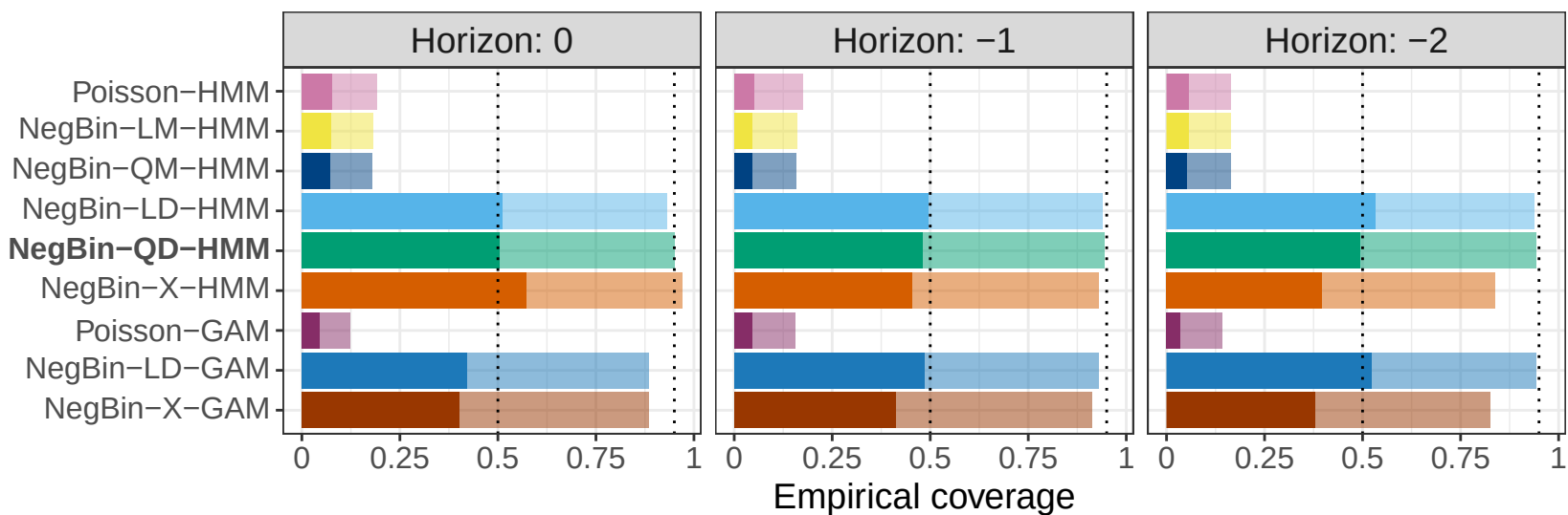
NegBin-QD data generating process
