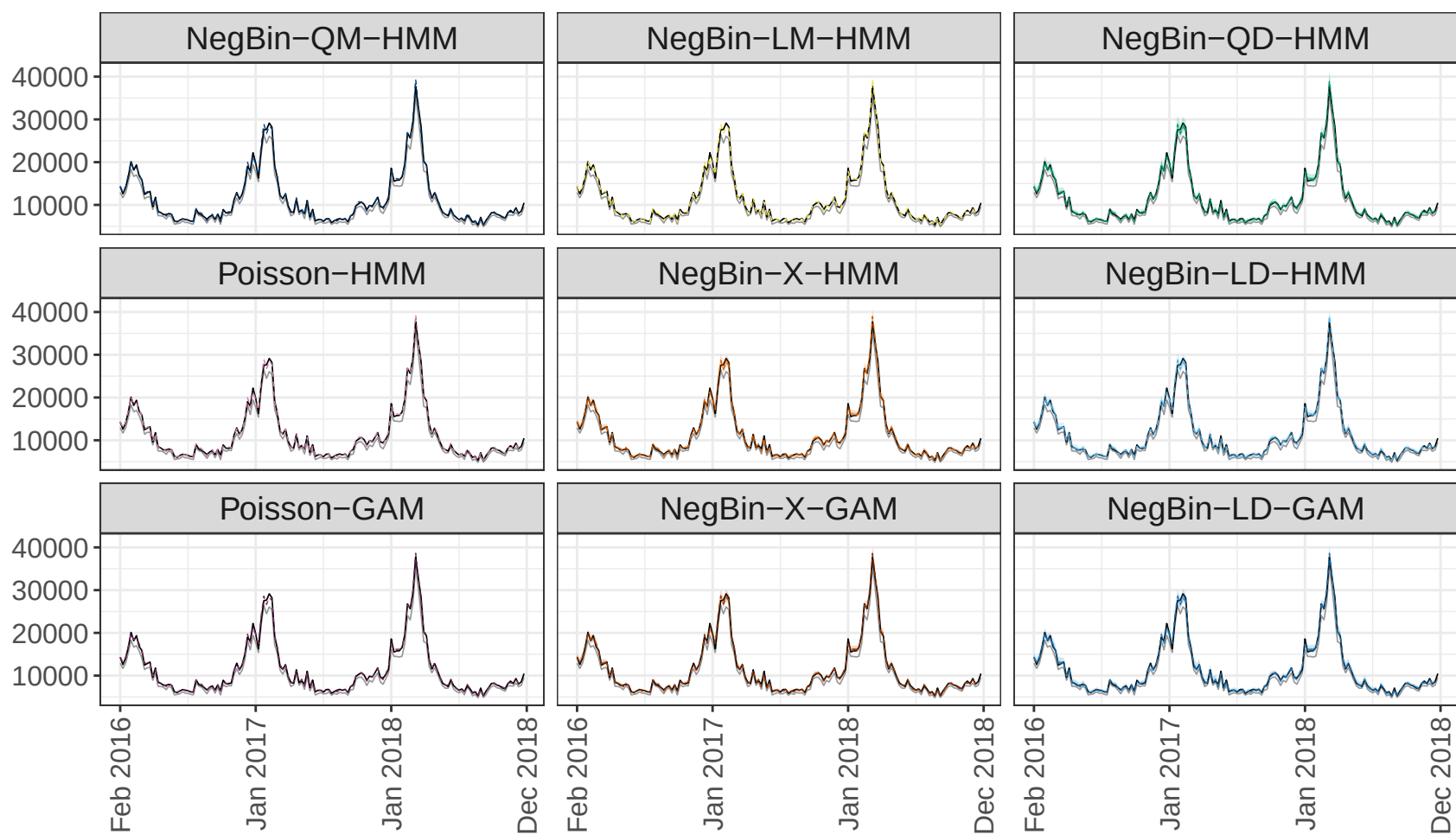
Horizon: -2 weeks
