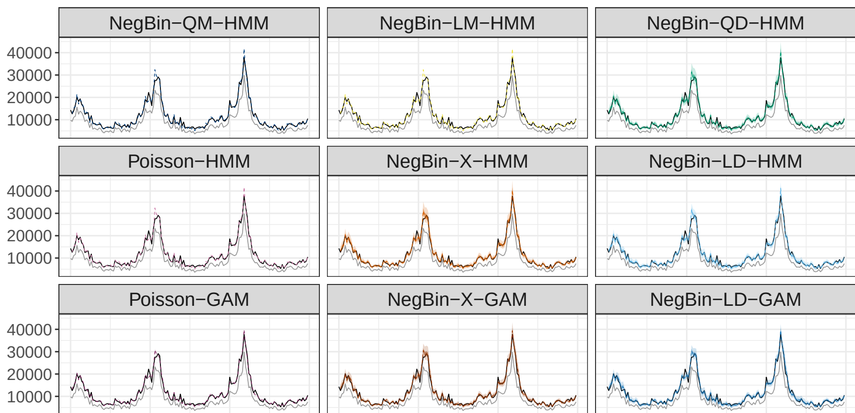
Horizon: -2 weeks
