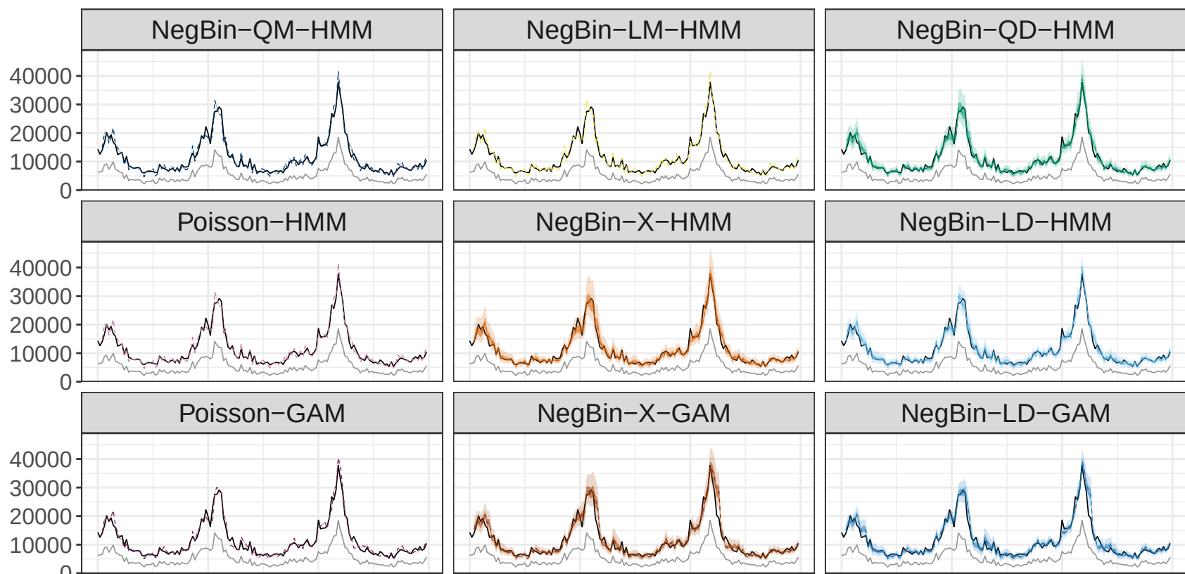
Horizon: -1 weeks
