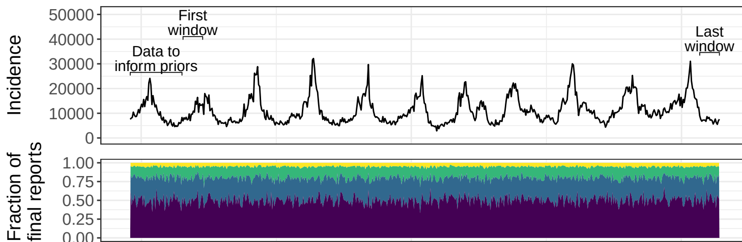
NegBin-LD data generating process
