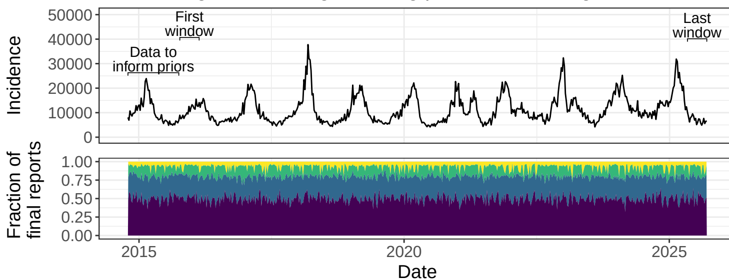
NegBin-X data generating process with irregularities
