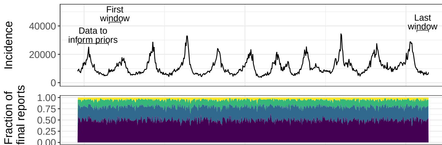
NegBin-X data generating process with irregularities
