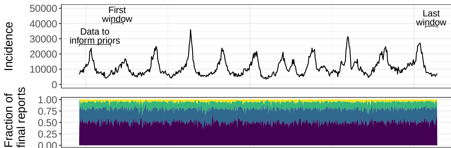
NegBin-QD data generating process
