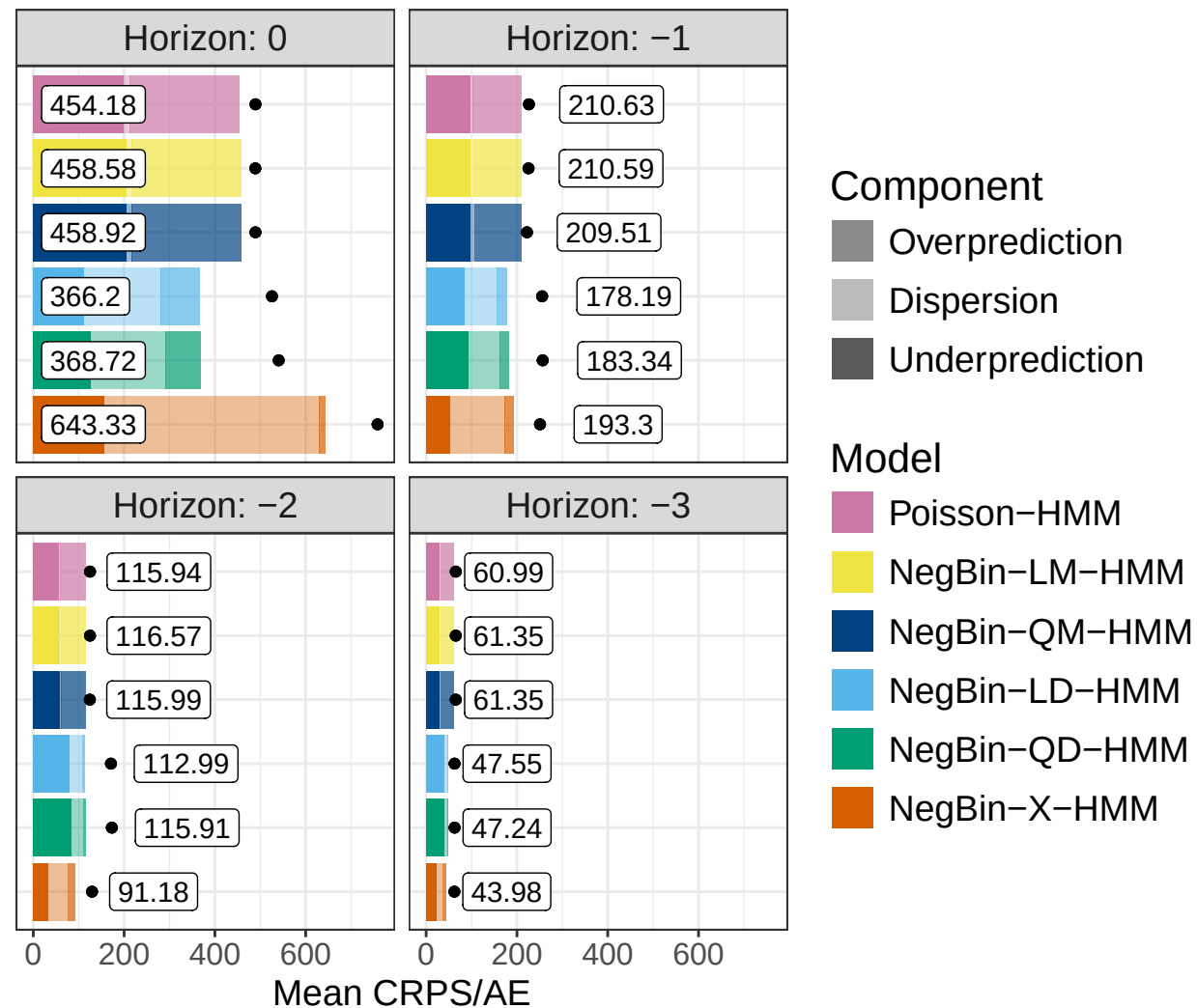
Stronger prior
