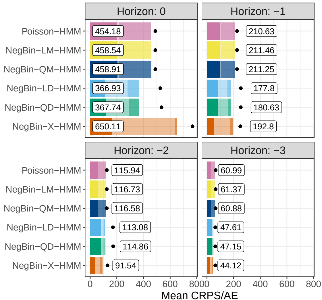
Weaker prior
