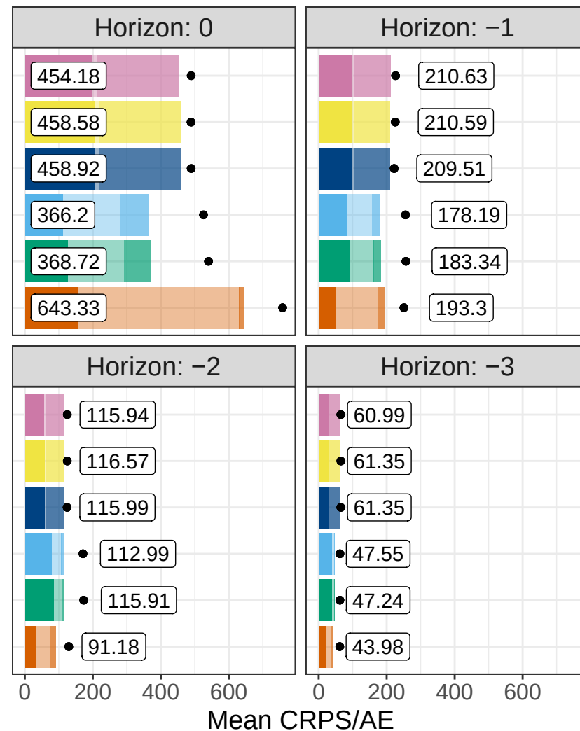
Stronger prior
