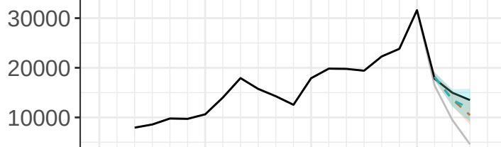
Nowcasts on 07 Apr 2019
