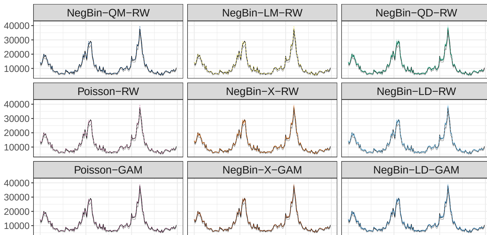
Horizon: -2 weeks
