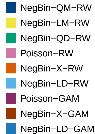
Model
