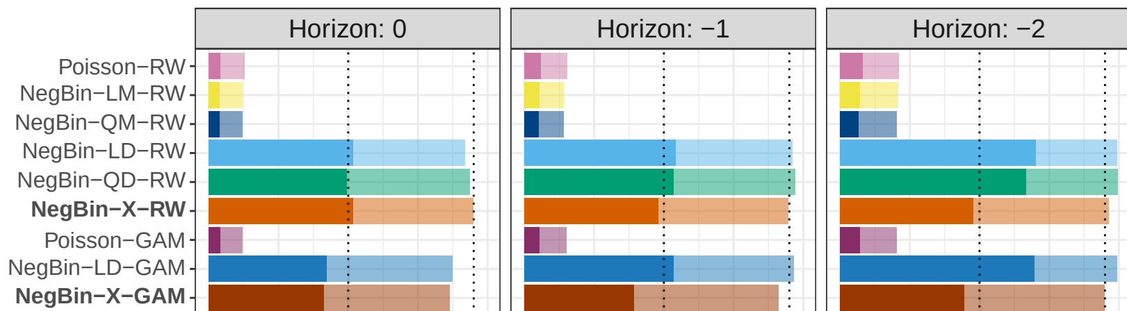
NegBin-LD data generating process
