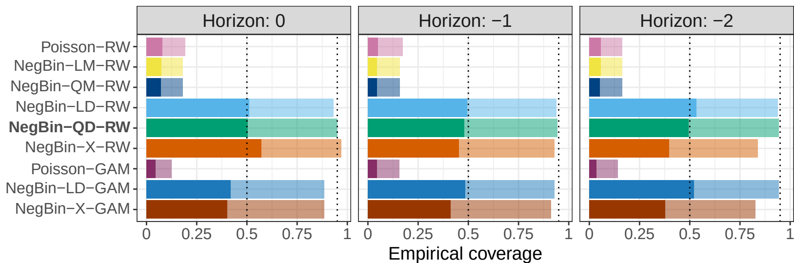
NegBin-QD data generating process
