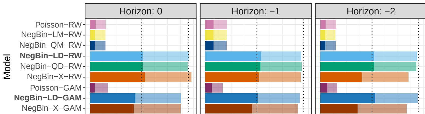
NegBin-QD data generating process
