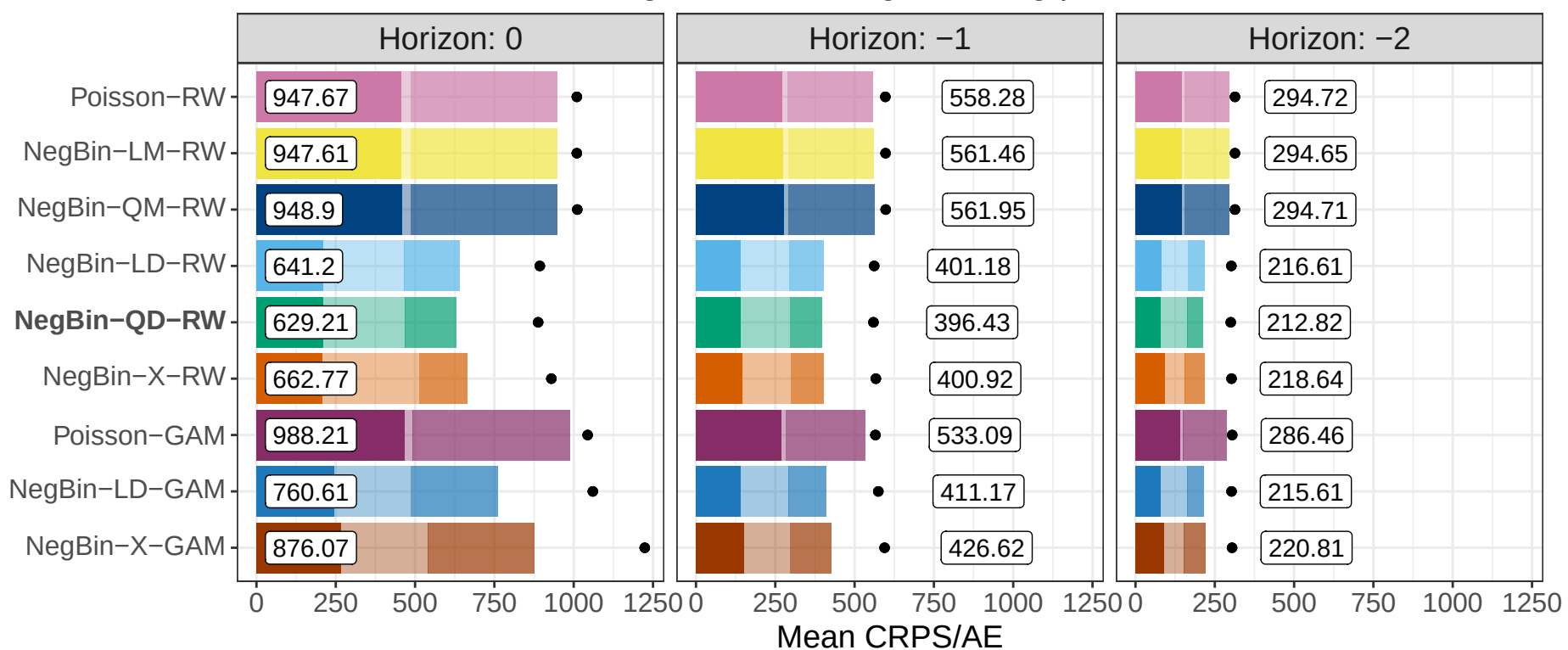
NegBin-QD data generating process
