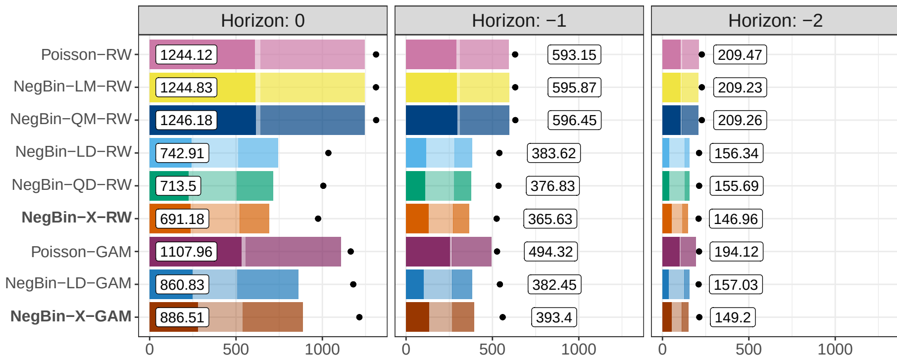
NegBin-LD data generating process
