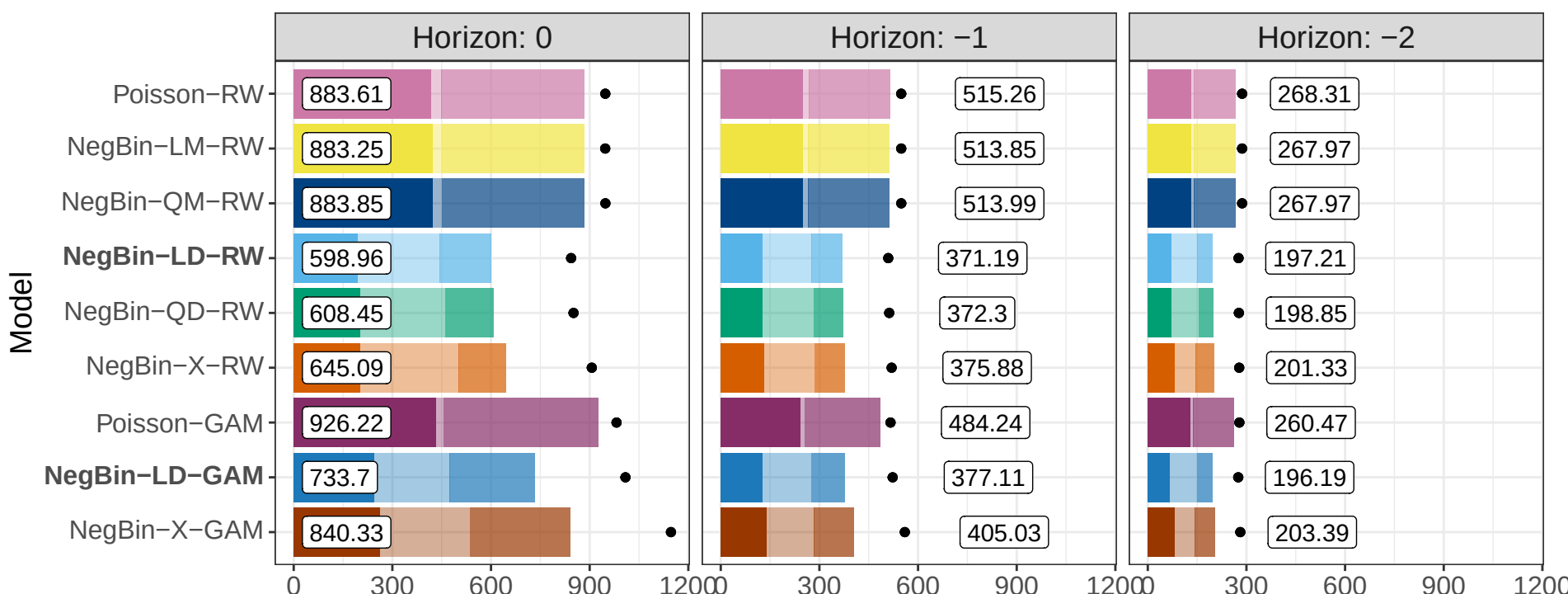
NegBin-QD data generating process
