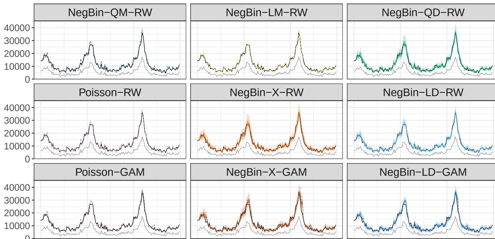
Horizon: -1 weeks
