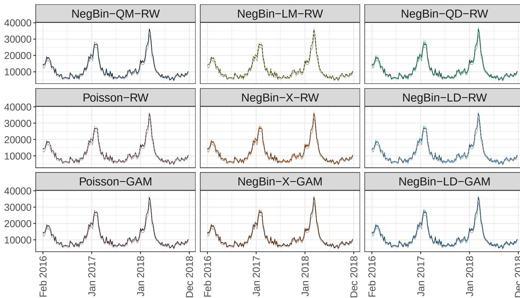
Horizon: -2 weeks
