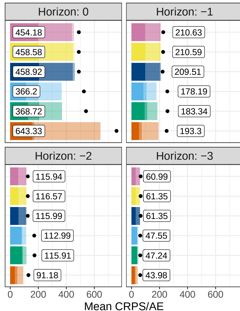
Stronger prior
