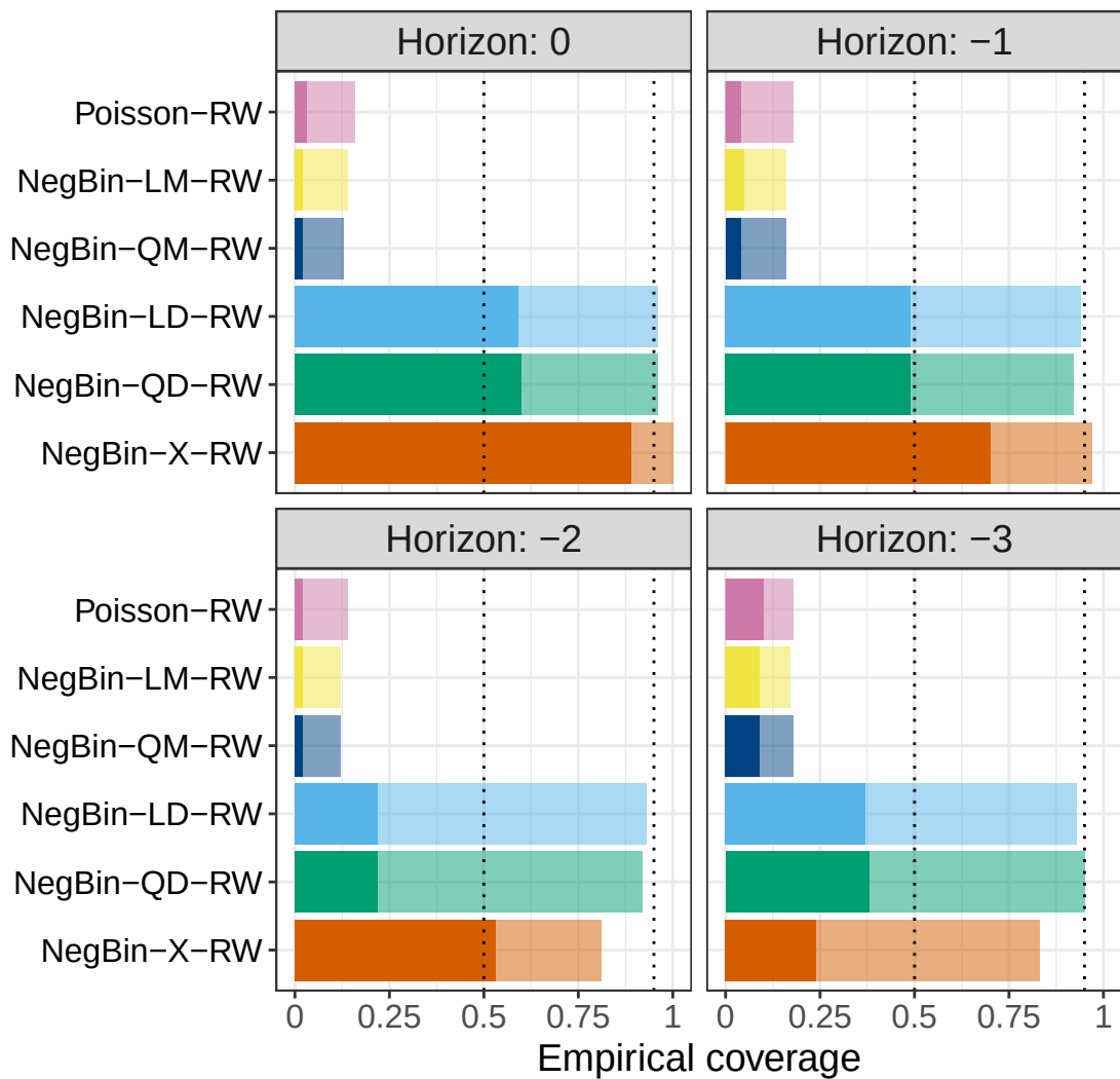
Weaker prior
