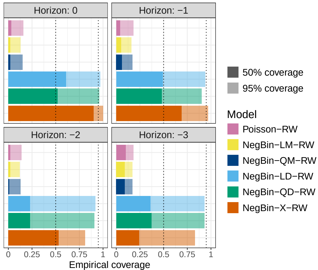
Stronger prior
