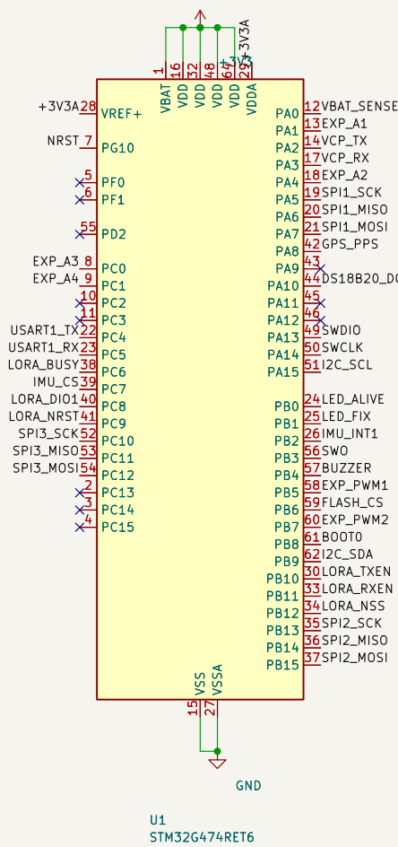
U1 STM32G474RET6
