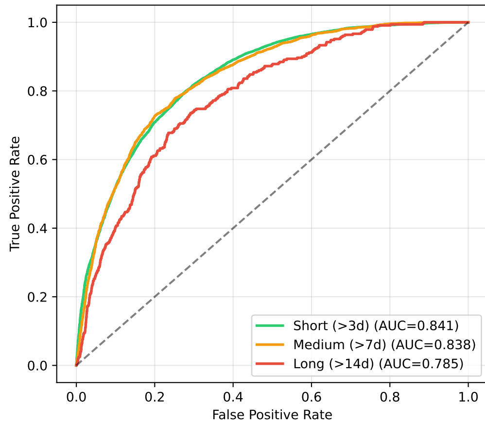
ROC Curves
