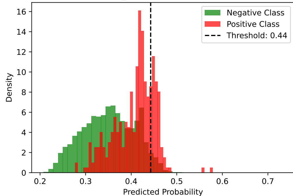
target_long Score Distribution
