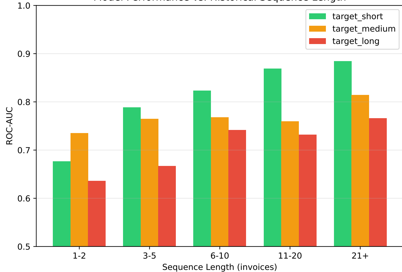
Model Performance vs. Historical Sequence Length
