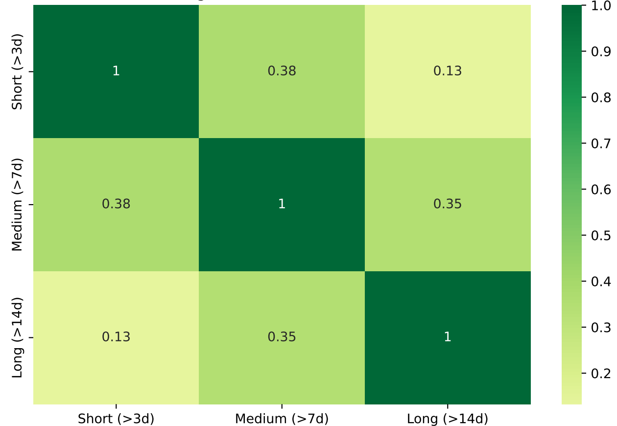
Target Variables Correlation
