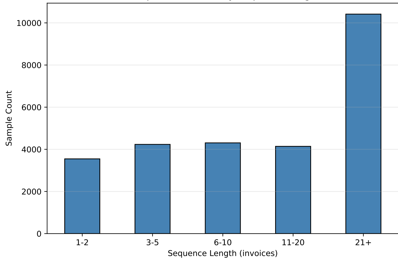
Sample Distribution by Sequence Length
