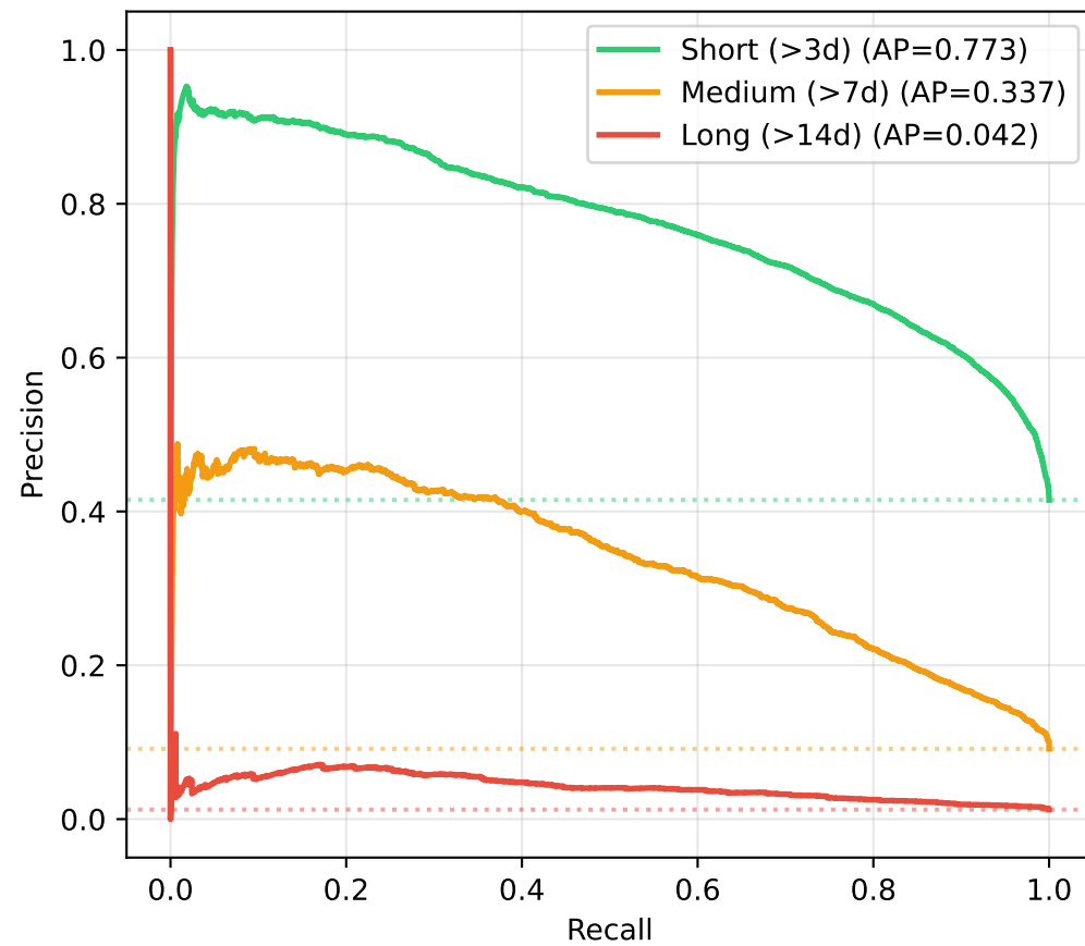
Precision-Recall Curves
