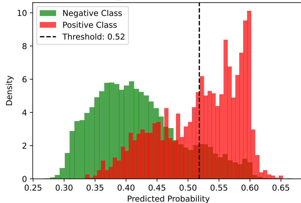
target_medium Score Distribution
