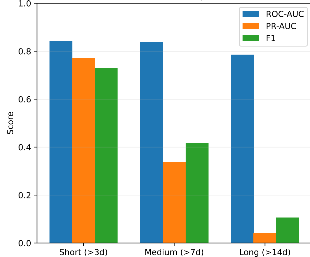
Performance Comparison
