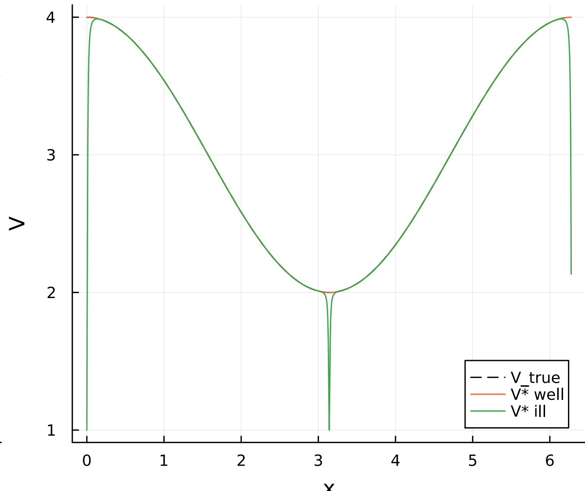
recovered V Adam
