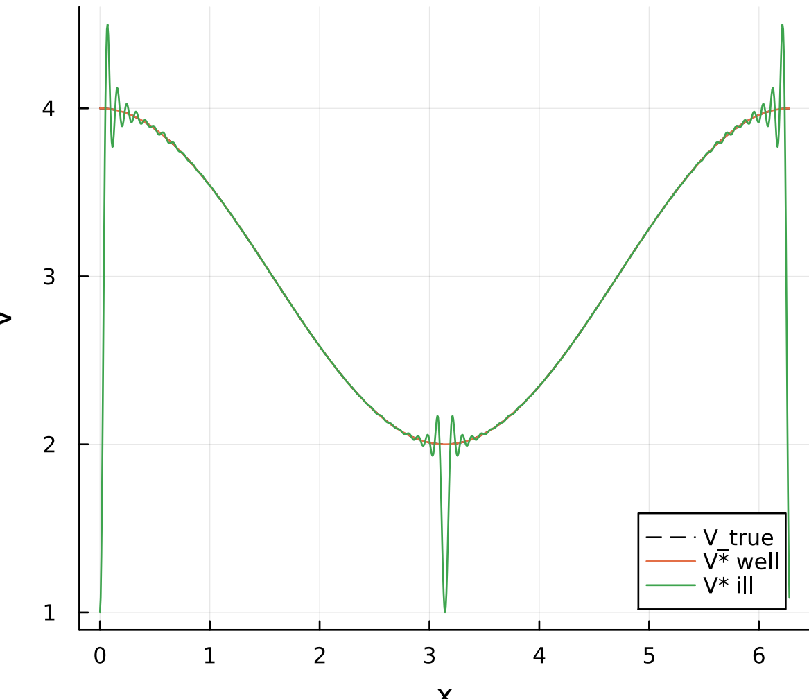
recovered V L-BFGS
