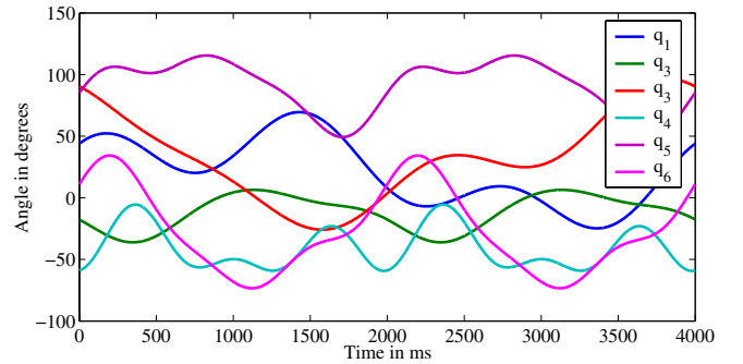
Fig. 5. Sinusoidal joint angles of trajectory T_2 .
