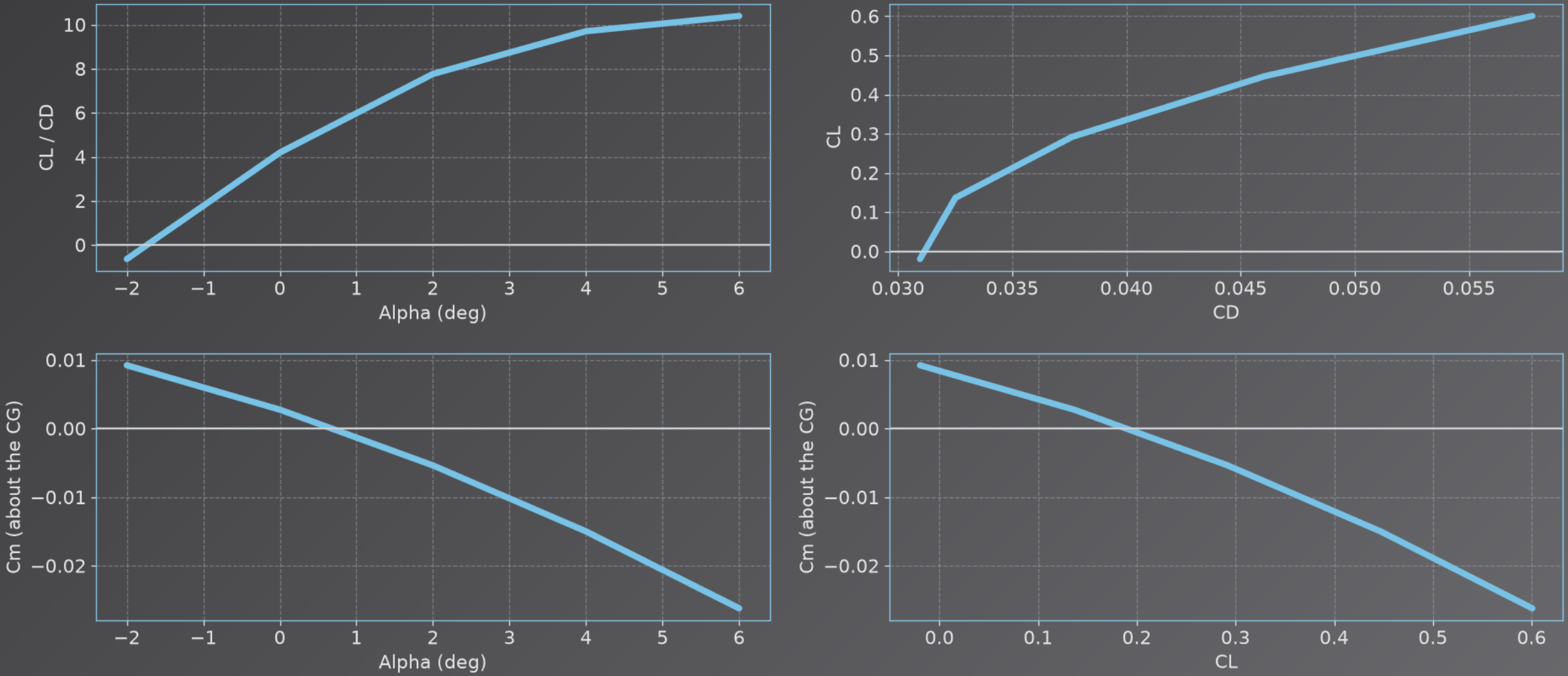
Whole aircraft, VSPAERO vortex lattice with the fuselage panels; best L/D 10.4 at 6.0°; Cm about the design CG.
