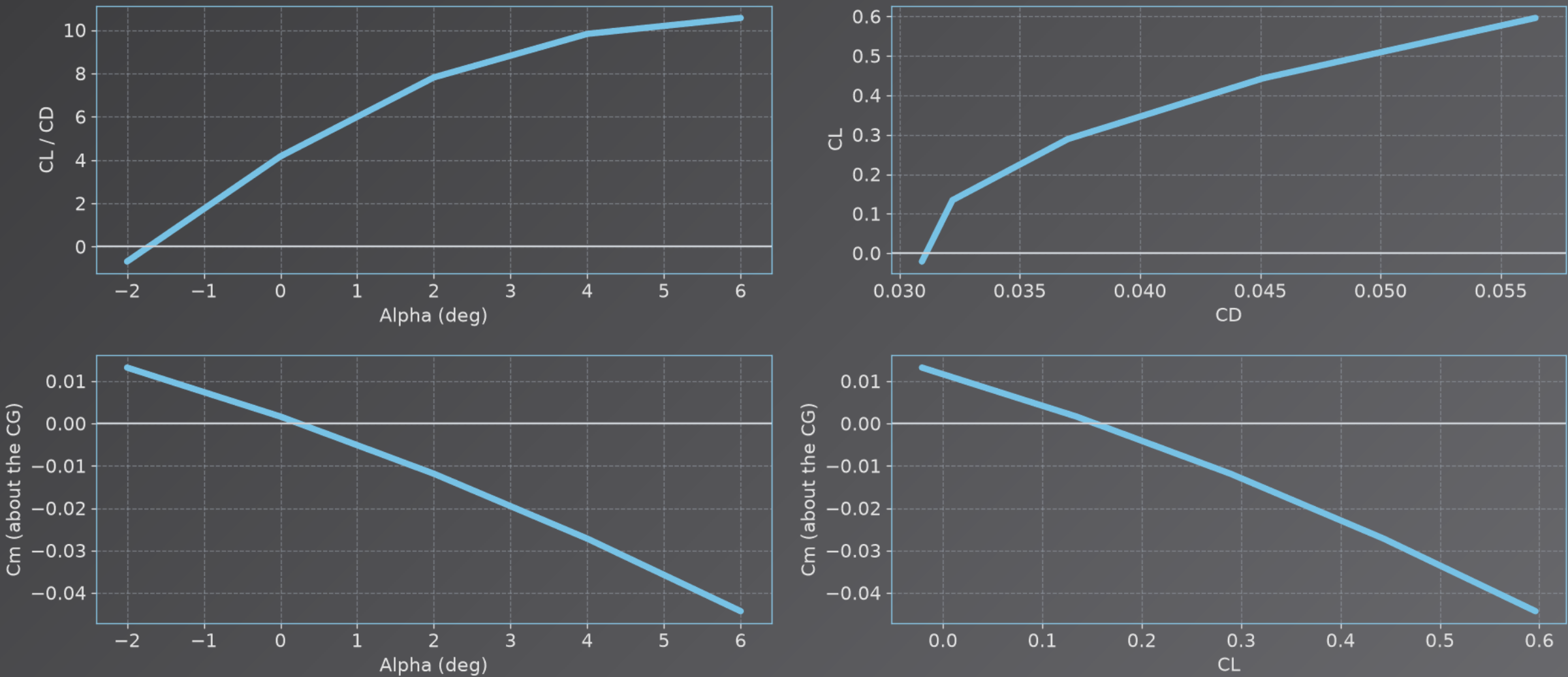
Whole aircraft, VSPAERO vortex lattice with the fuselage panels; best L/D 10.6 at 6.0^\circ ; C_m about the design CG.
