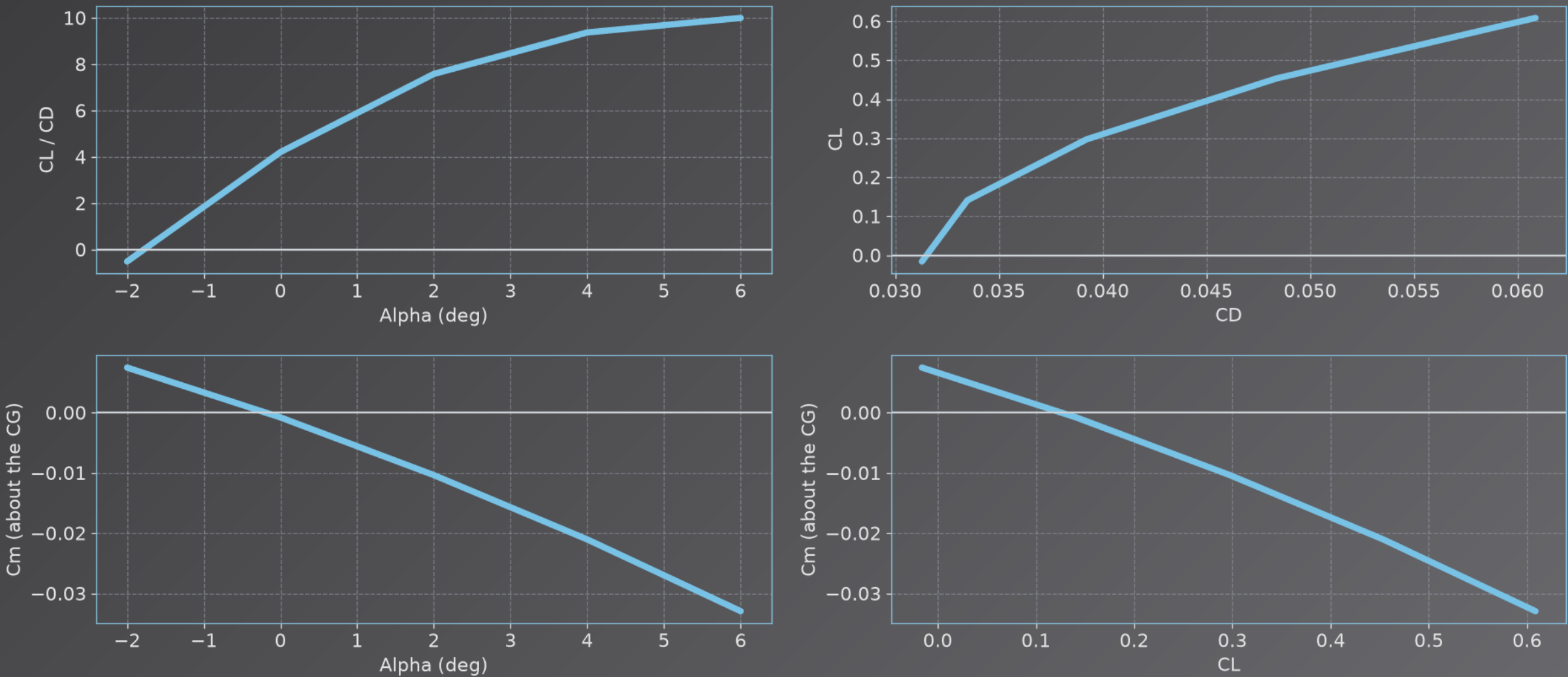
Whole aircraft, VSPAERO vortex lattice with the fuselage panels; best L/D 10.0 at 6.0°; C_m about the design CG.
