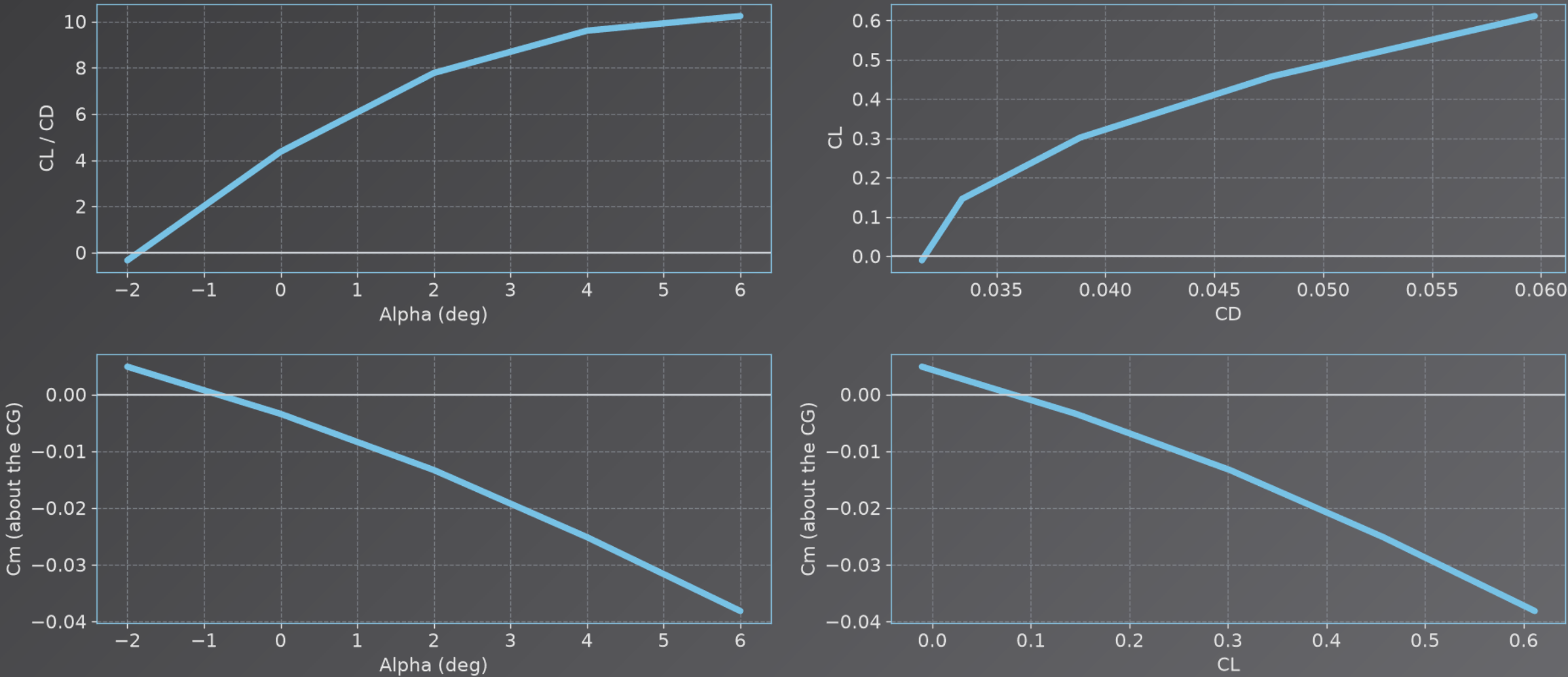
Whole aircraft, VSPAERO vortex lattice with the fuselage panels; best L/D 10.2 at 6.0^\circ ; C_m about the design CG.
