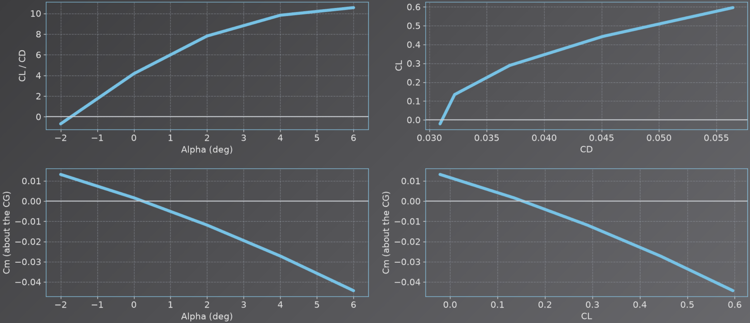
Whole aircraft, VSPAERO vortex lattice with the fuselage panels; best L/D 10.6 at 6.0°; C_m about the design CG.
