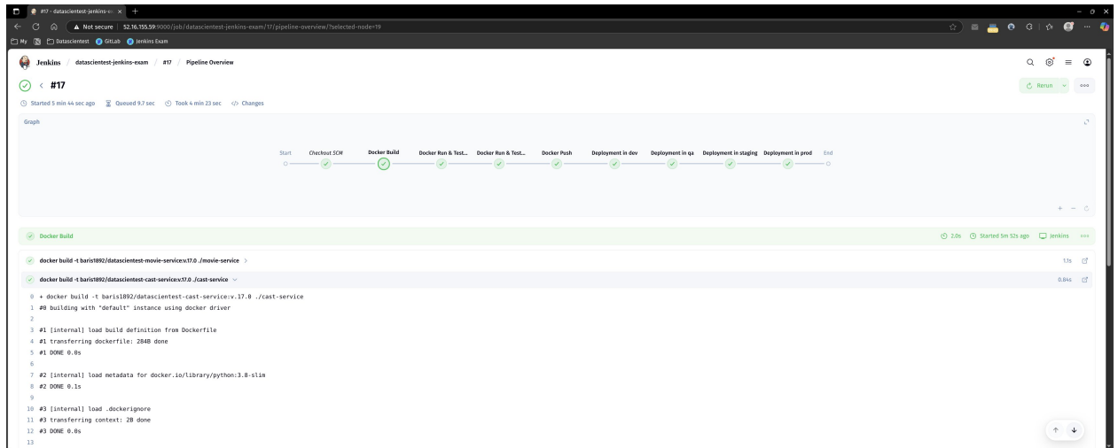
Figure 1: Docker Build
