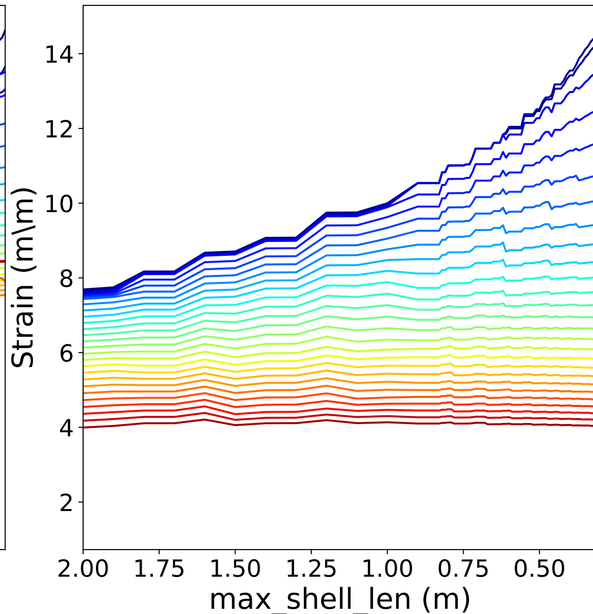
Strain at multiple distances from point load at A in direction West
