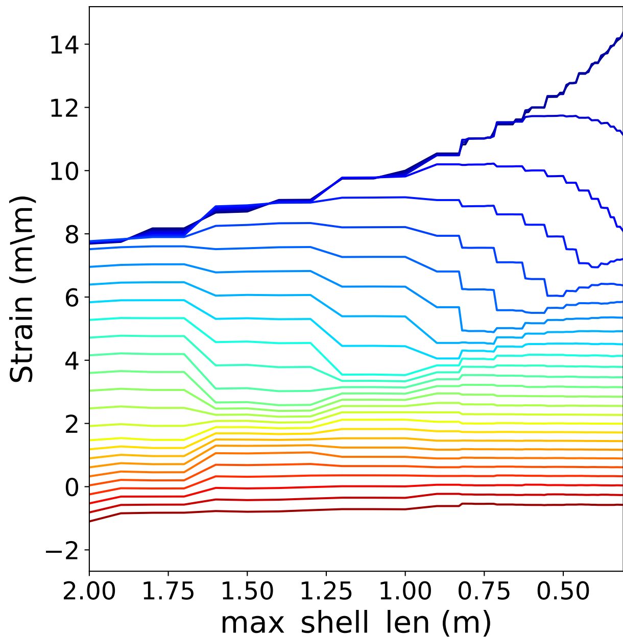
Strain at multiple distances from point load at A in direction East
