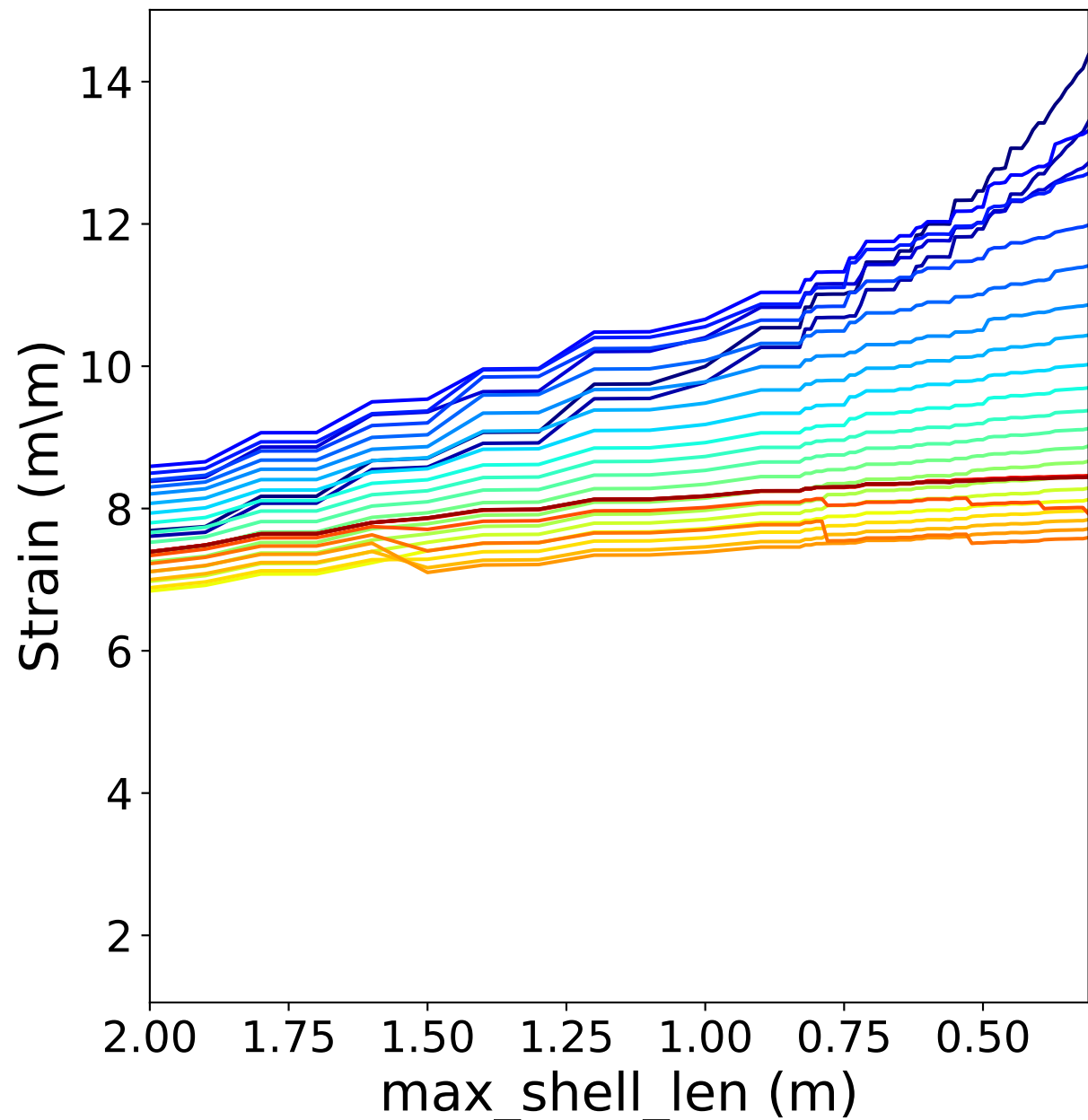
Strain at multiple distances from point load at A in direction East
