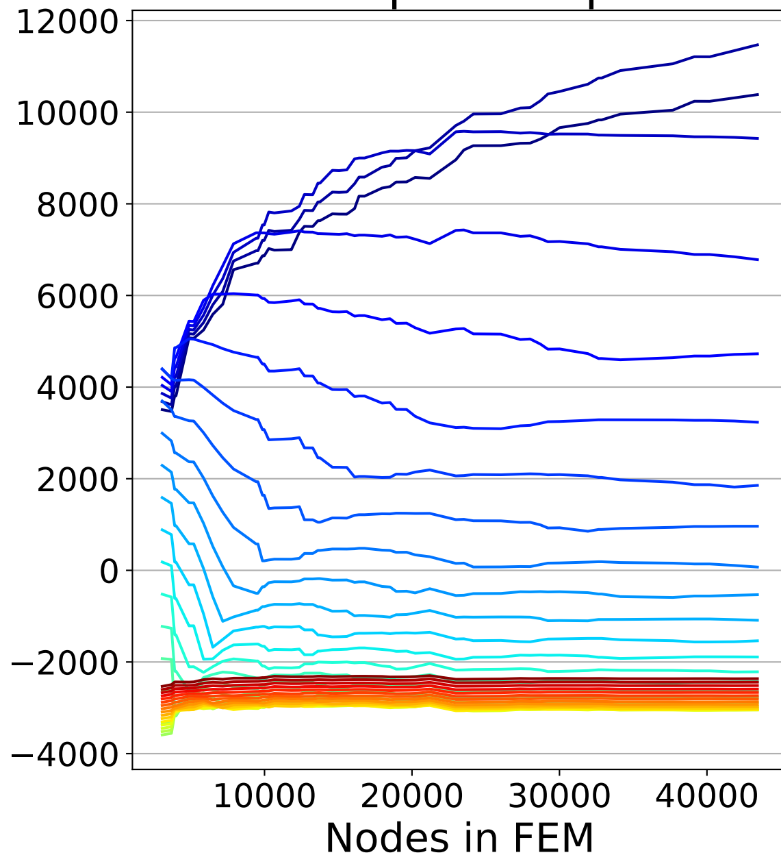
Strain at increasing distance in direction West from the NW point of pier 5
