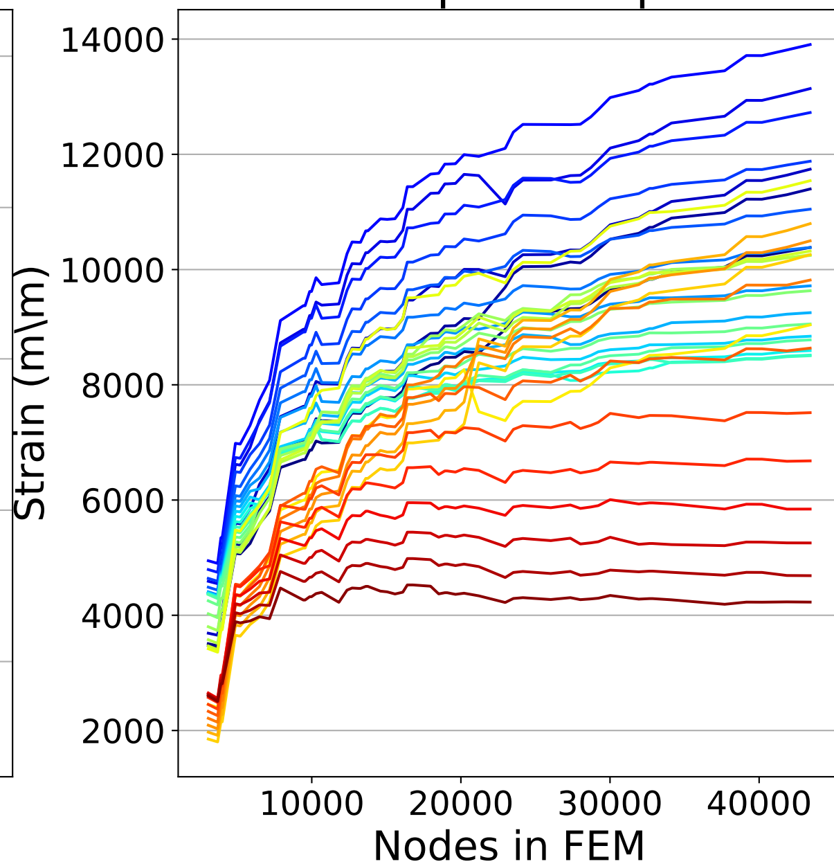
Strain at increasing distance in direction West from the NW point of pier 5
