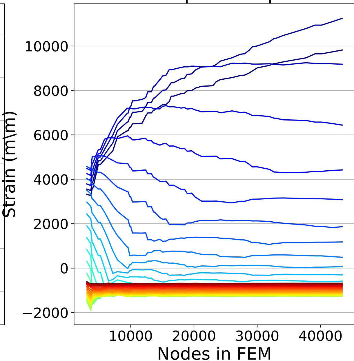
Strain at increasing distance in direction West from the NW point of pier 4
