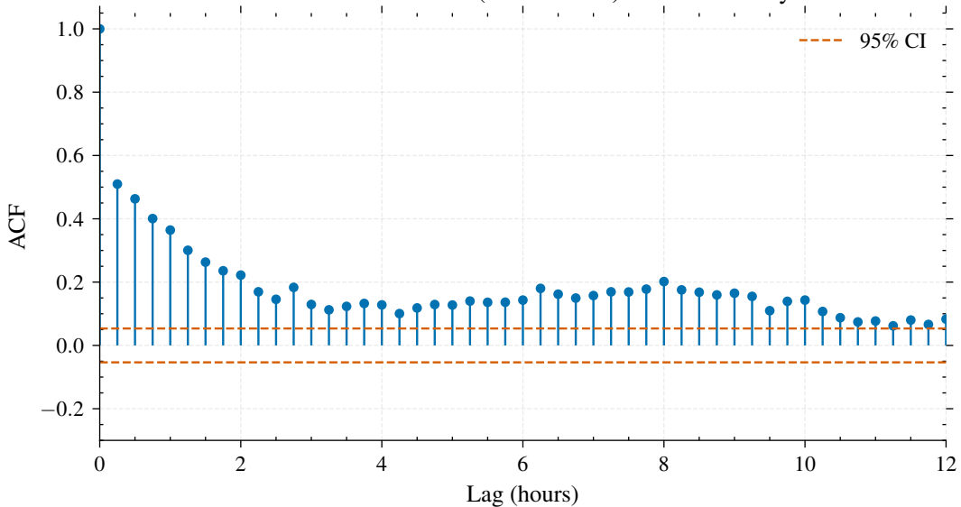
ACF of Event Counts (15-min bins) — First 14 Days
