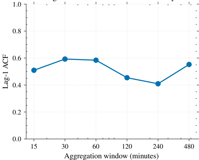
Lag-1 ACF vs Window — First 14 Days
