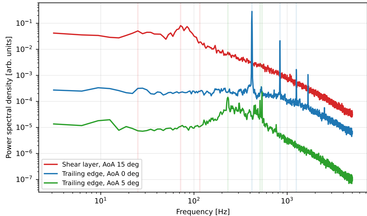
HWA energy spectra
