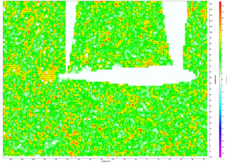
DaVis window-size test 16 x 16 px
