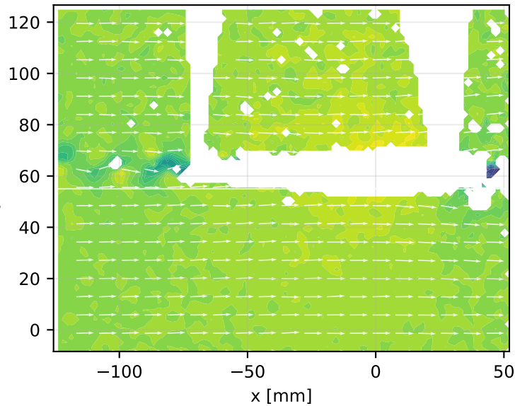
Instantaneous PIV field, AoA 0 deg
