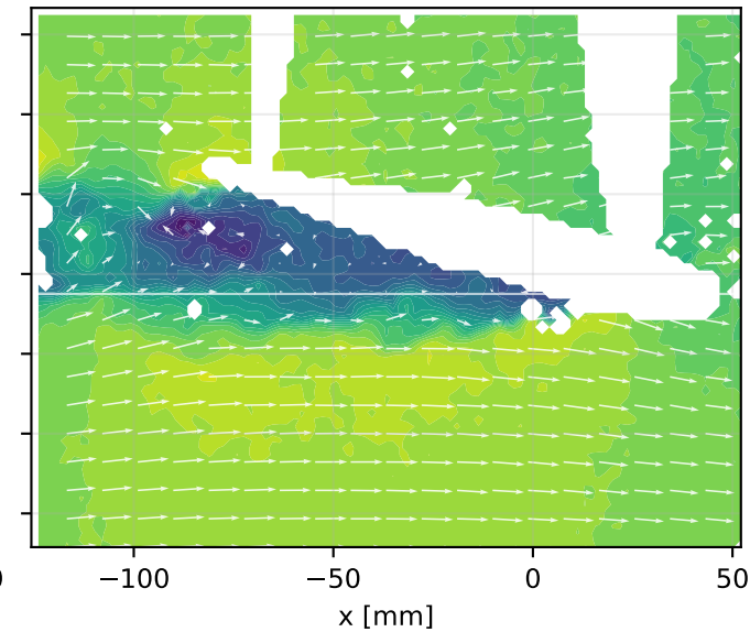
Instantaneous PIV field, AoA 15 deg
