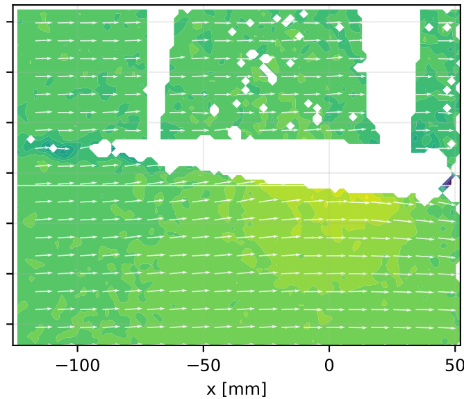
Instantaneous PIV field, AoA 5 deg
