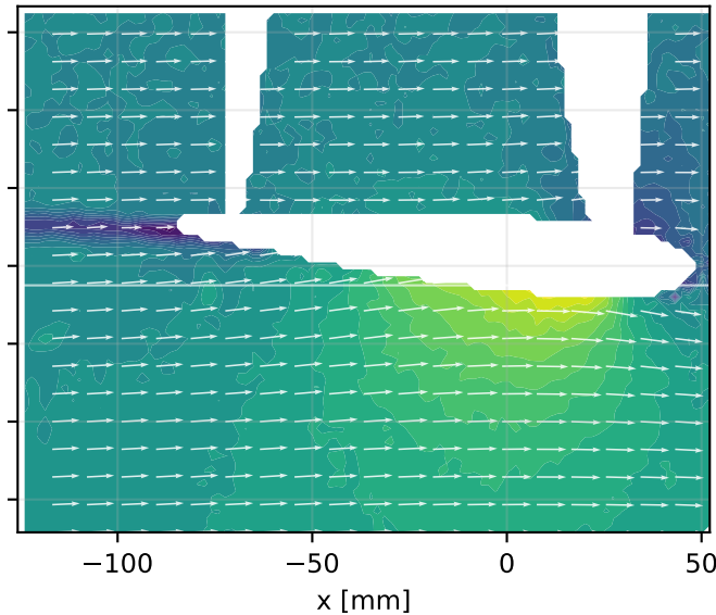
Mean PIV field, AoA 5 deg
