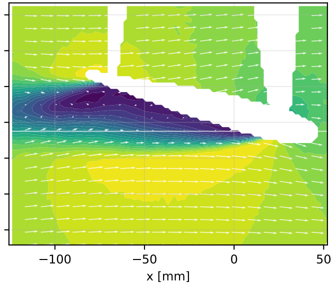
Mean PIV field, AoA 15 deg
