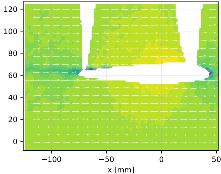
Mean PIV field, AoA 0 deg
