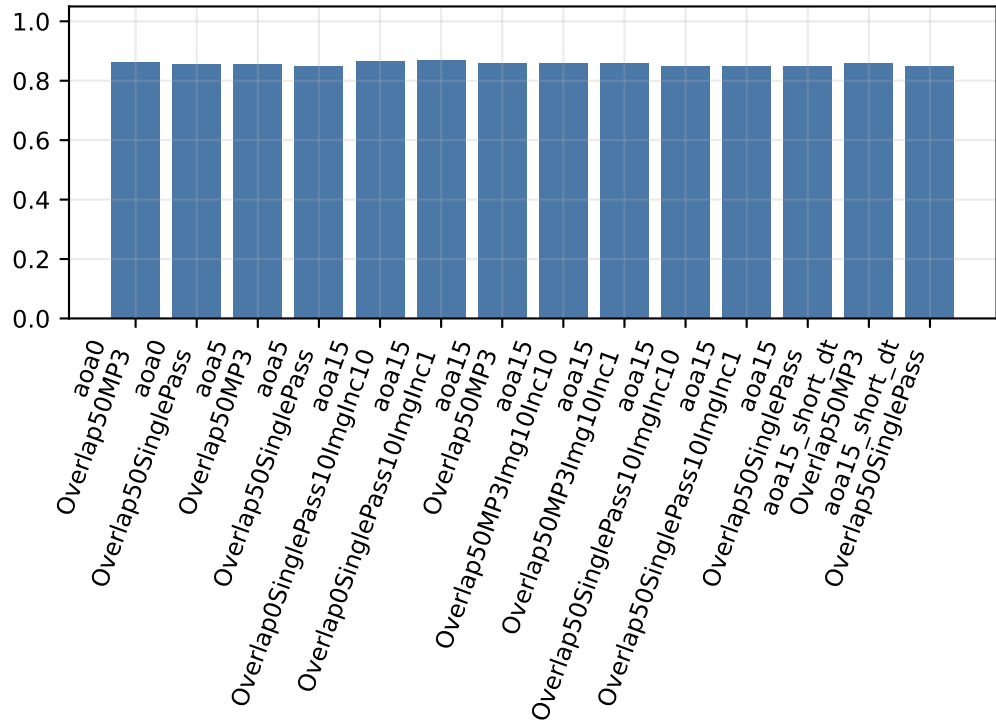
Valid-vector fraction
